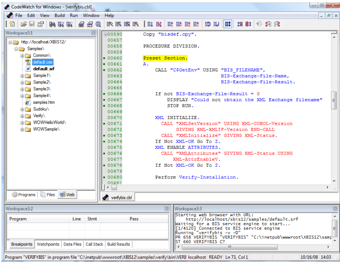
Figure 8. CodeWatch debugging a BIS application
