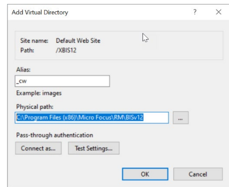
Figure 24. IIS Add Virtual Directory Dialog Box.
