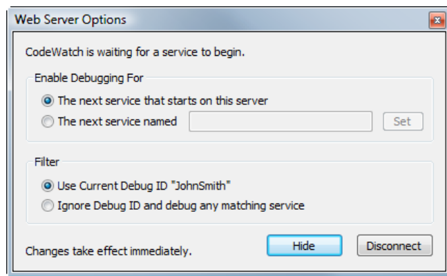
Figure 22. Web Server Options Dialog
