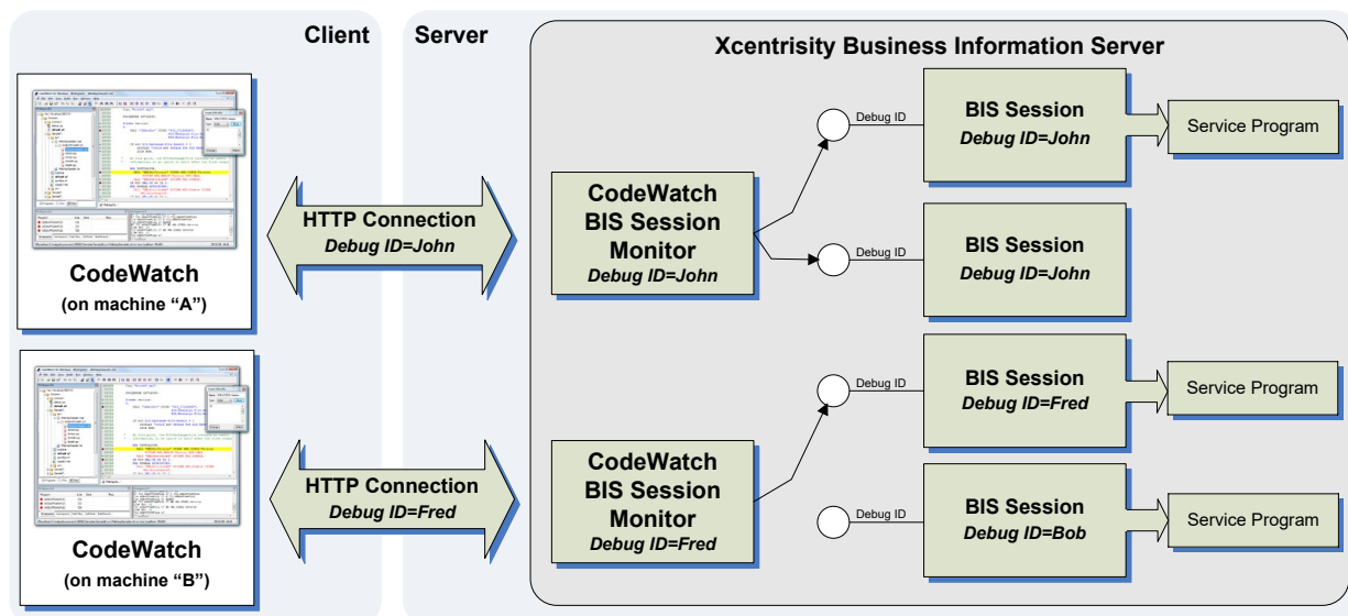
Figure 10. CodeWatch for BIS Control Flow
