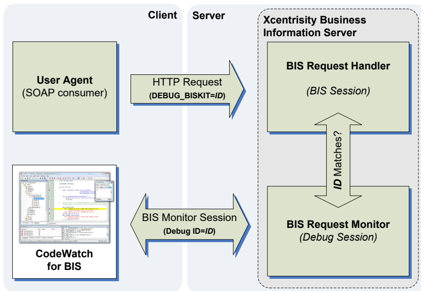
Figure 21. Web Services Debugging
