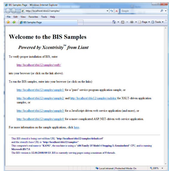
Figure 2. BIS Samples in Internet Explorer
