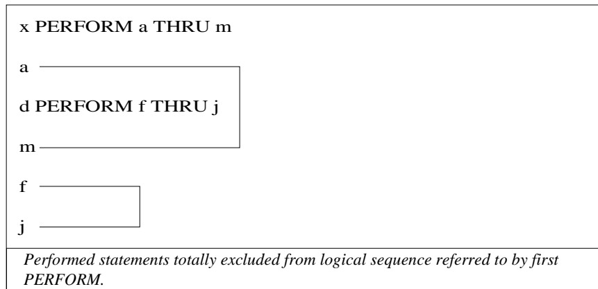
Figure 11: PERFORM Statement Examples
