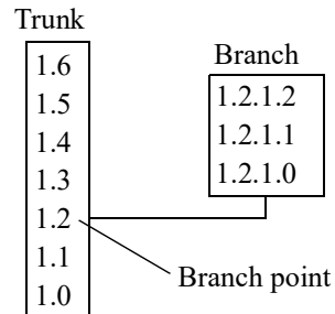
Figure 15-1. Branching
