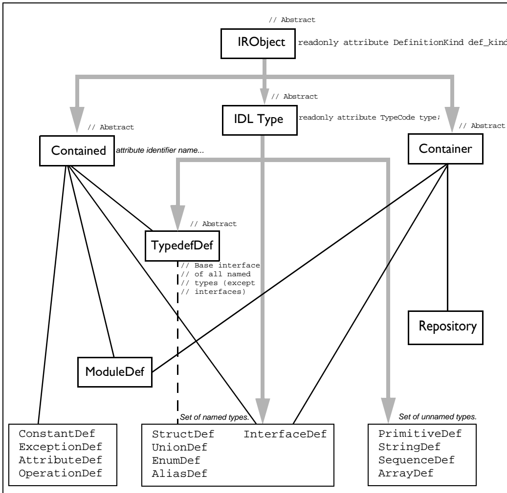
Figure 15.1: The Hierarchy for Interface Repository Interfaces
