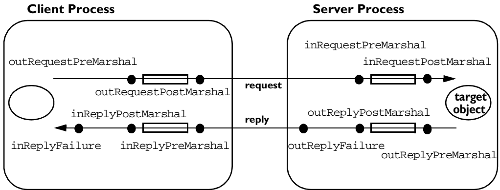
Figure 16.2: Per-process Monitor Points
