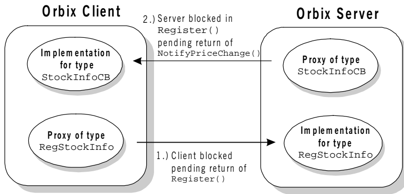
Figure 18.4: Deadlock in a Callback Model
