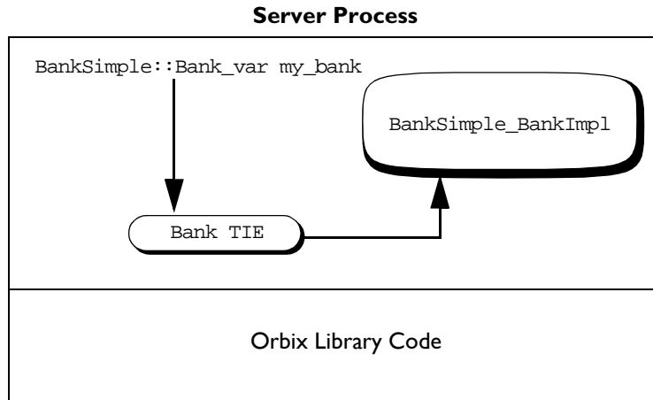
Figure 5.3: State of the Server at Launch
