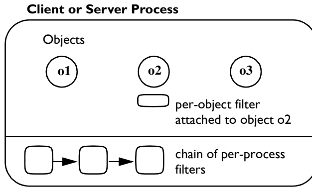
Figure 16.1: Per-process and Per-object Filtering
