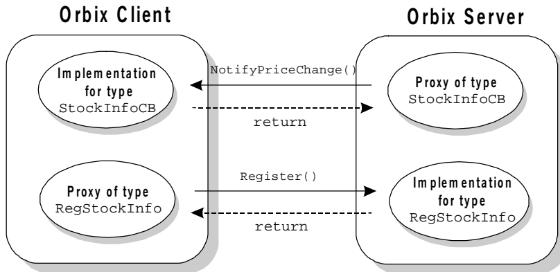
Figure 18.3: Client-Server Callback Interaction
