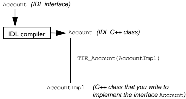
Figure 5.2: The TIE Approach to Implementing Interfaces
