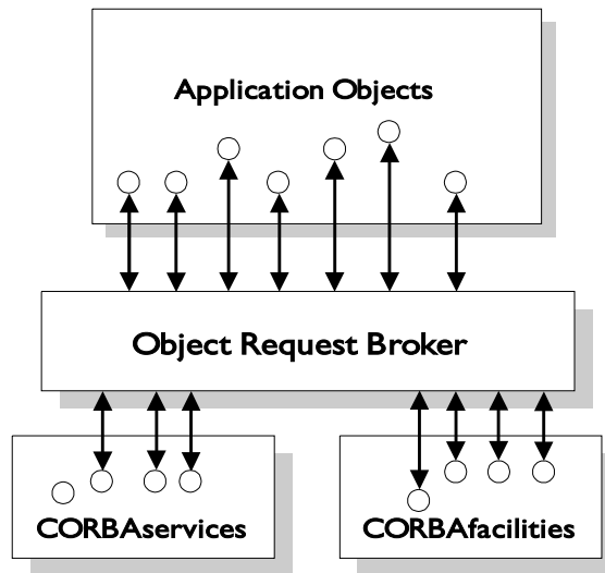
Figure I.5: The Object Management Architecture
