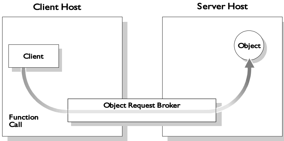
Figure 1.1: The Object Request Broker
