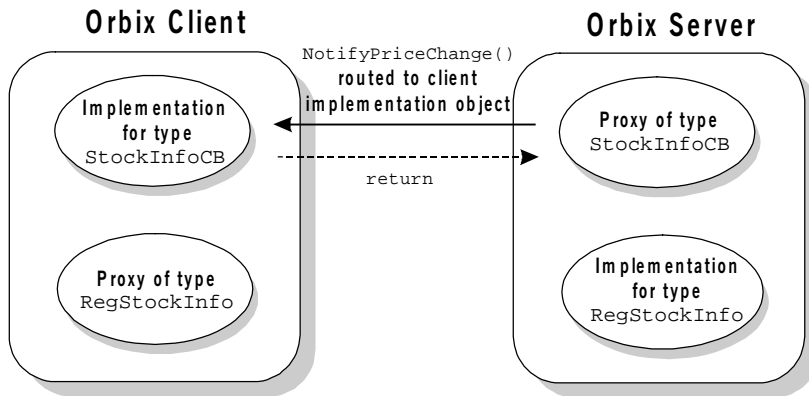
Figure 18.2: Server Invoking Operation on Client Callback Object
