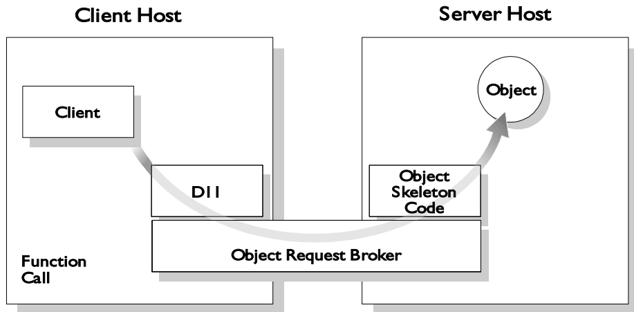
Figure 1.3: Client Invoking a Function Using the DII
