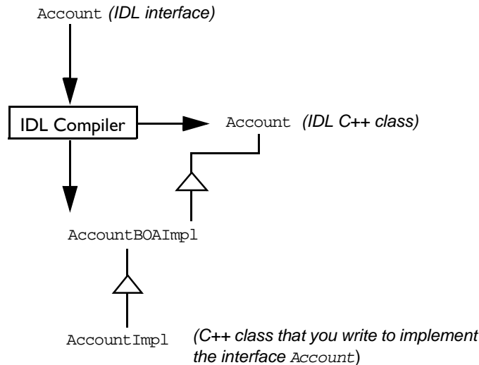
Figure 5.1: The BOAImpl Approach to Defining a C++ Implementation Class
