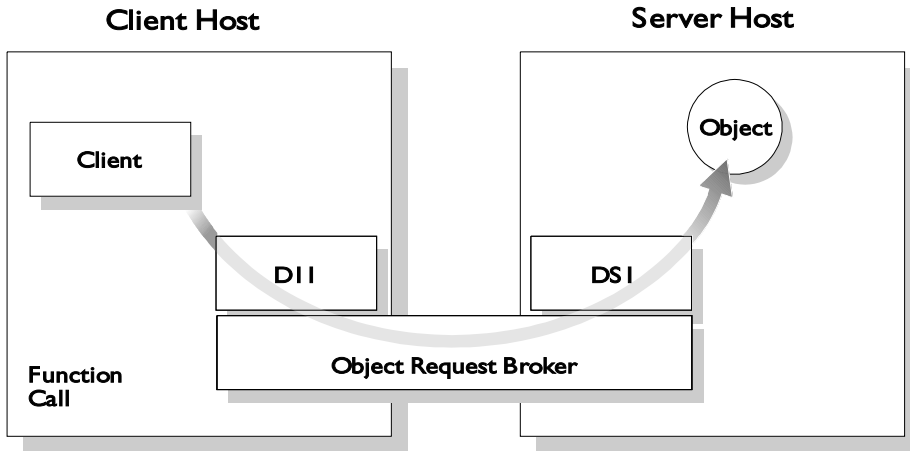
Figure 1.4: Function Call Using the DII and DSI
