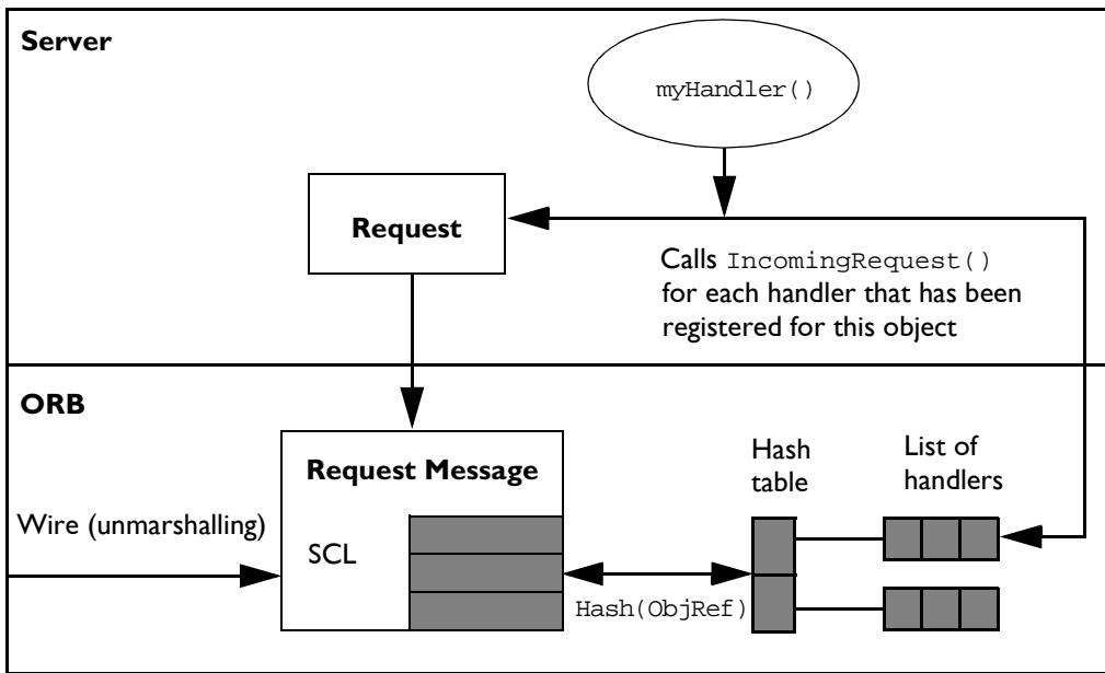
Figure 24.4: Service Contexts Per Object: Server Side
