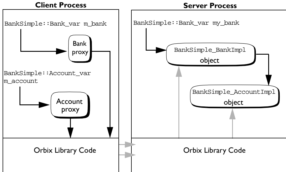
Figure 5.6: Client Accesses Account Object (BOAImpl Approach)
