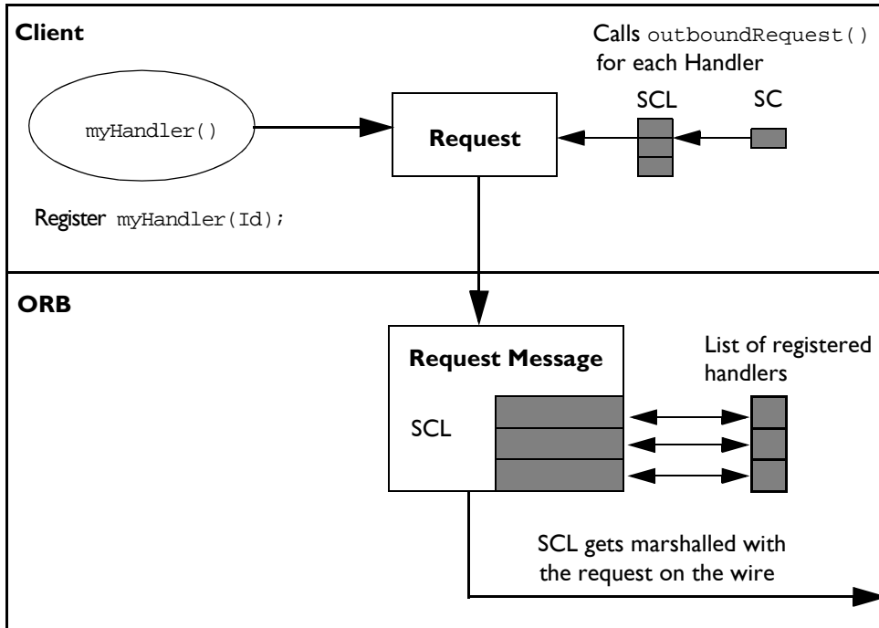
Figure 24.1: Service Contexts Per Request: Client Side
