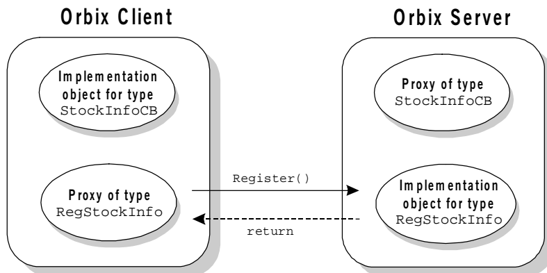
Figure 18.1: Client Passes Implementation Object Reference to Server
