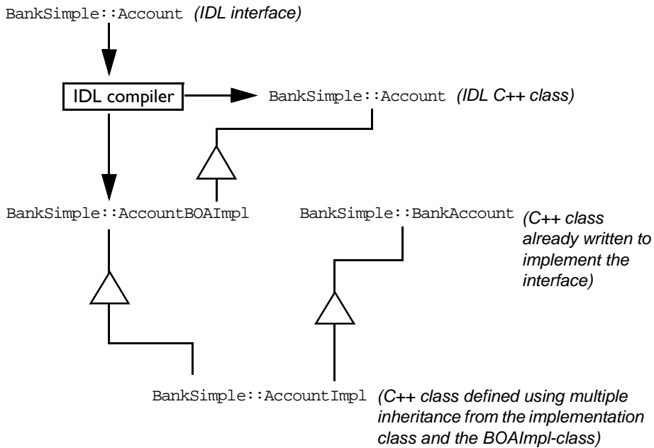
Figure 5.7: BOAImpl Approach to Allow an Existing Class to Implement an IDL Interface
