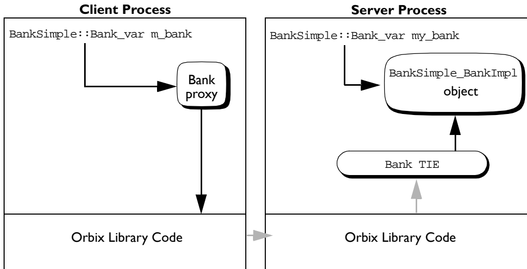
Figure 5.4: Client Binds to Bank Object (TIE Approach)
