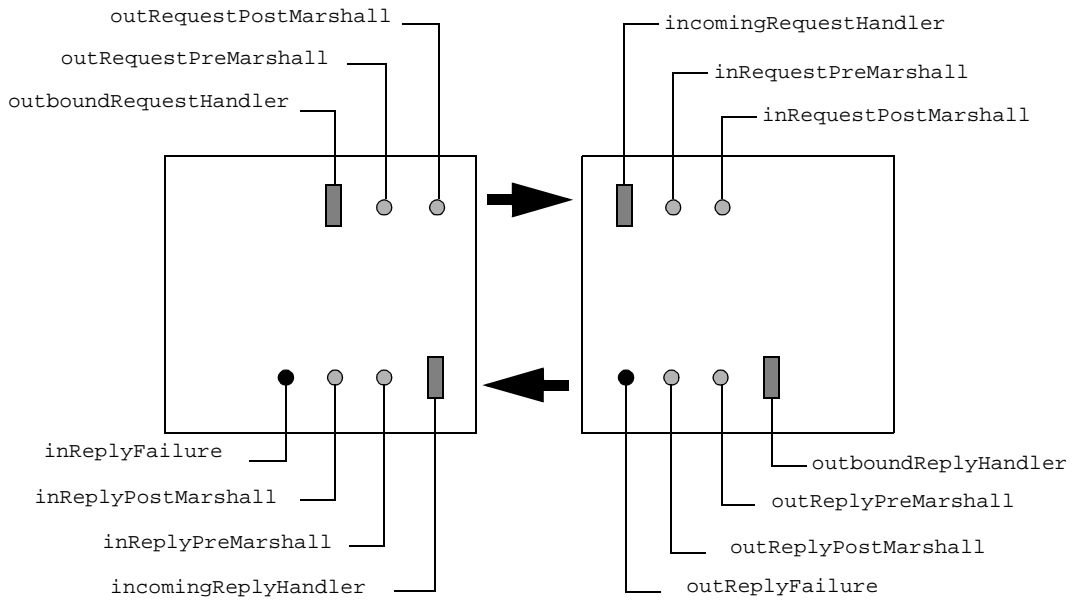
Figure 24.5: Service Context Handlers and Filter Points
