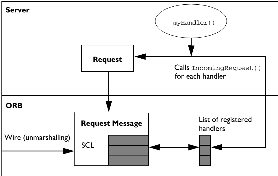
Figure 24.2: Service Contexts Per Request: Server Side
