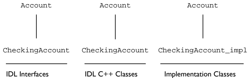
Figure 8.1: IDL and Corresponding C++ Class Hierarchies
