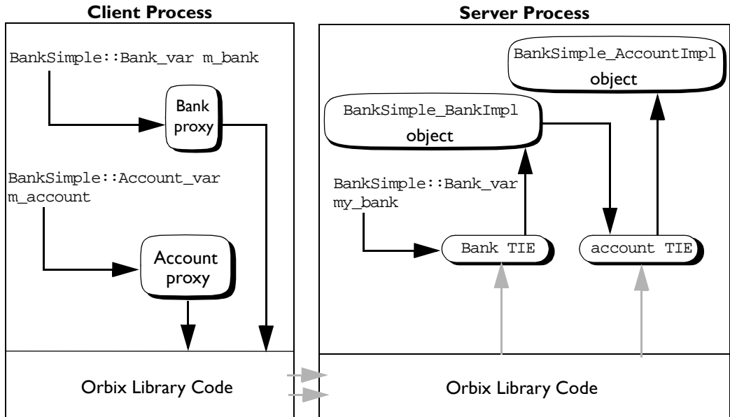
Figure 5.5: Client Accesses Account Object (TIE Approach)
