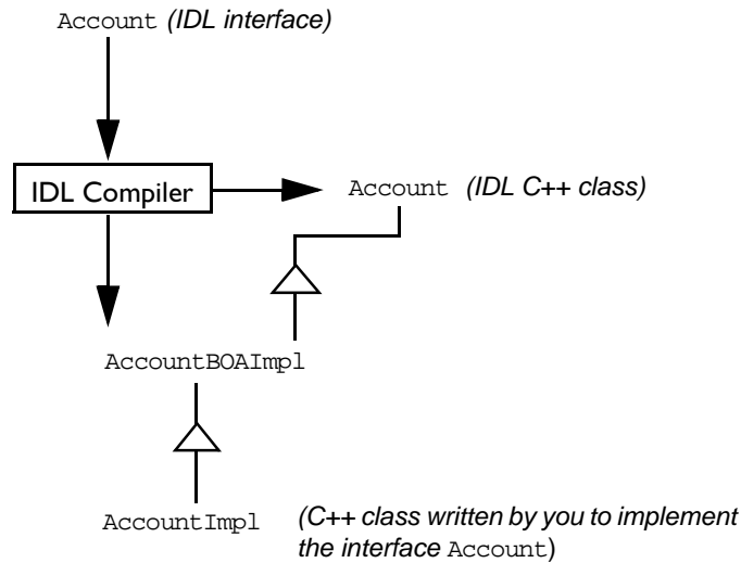
Figure 10.1: Casting From Interface Class to Implementation Class Using the BOAImpl Approach
