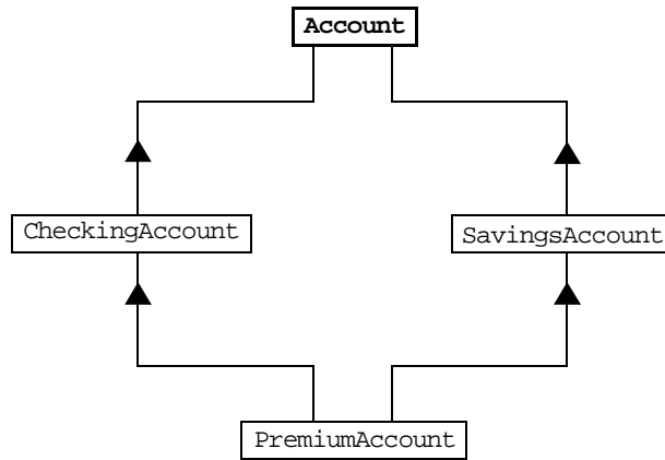
Figure 3.1: Multiple Inheritance of IDL Interfaces
