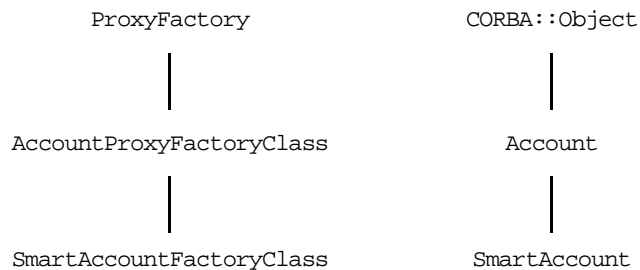
Figure 17.1: Class Hierarchy for Smart Proxy Class
