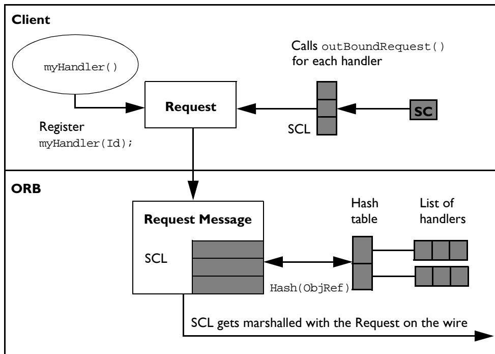
Figure 24.3: Service Contexts Per-Object: Client Side
