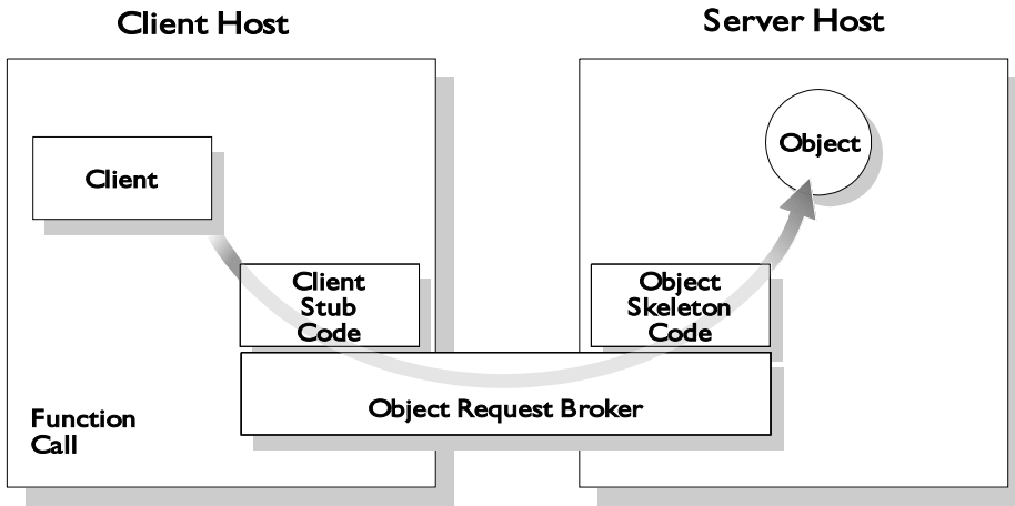
Figure 1.2: Invoking on a CORBA Object
