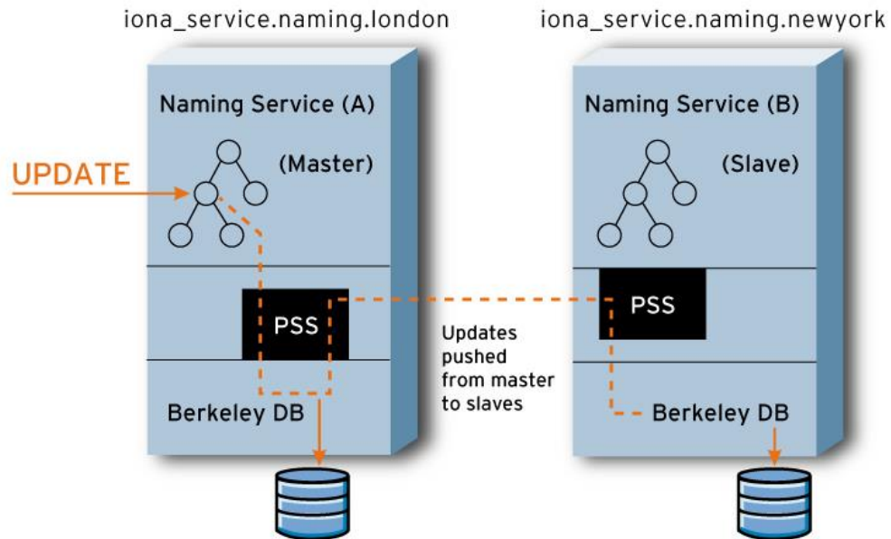
Figure 7: Orbix Replication
