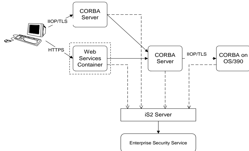
Figure 1: Orbix Security Framework Architecture
