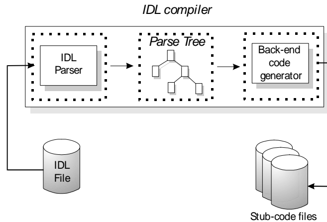
Figure 1: Standard IDL Compiler Components
