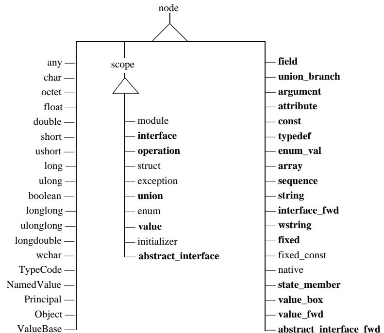
Figure 5: Inheritance Hierarchy for Node Types
