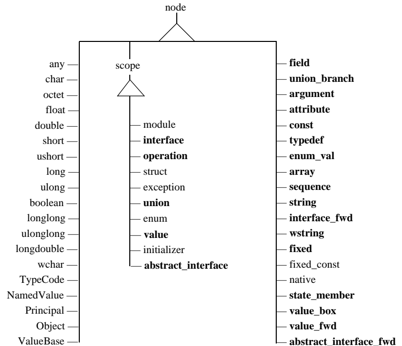
Figure 4: Inheritance Hierarchy for Node Types
