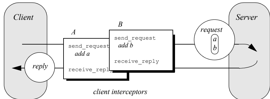
Figure 40 Client interceptors allow services to access outgoing requests and incoming replies.
