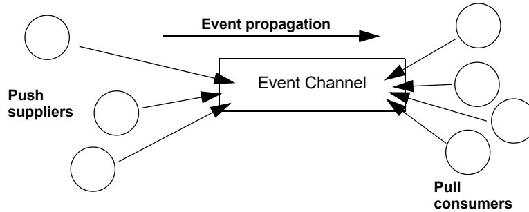
Figure 38 Push suppliers and pull consumers communicating through an event channel
