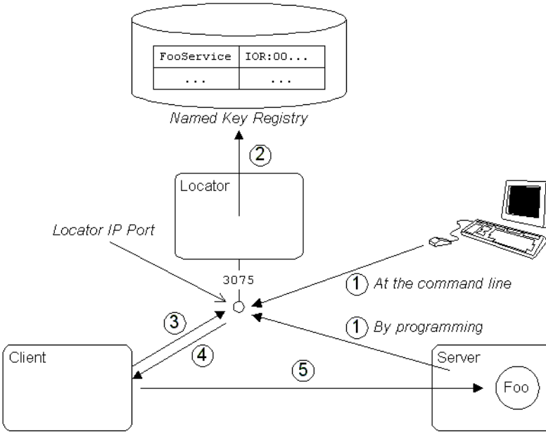
Figure 52 Using corbaloc with the Locator-Based Named Key Registry
