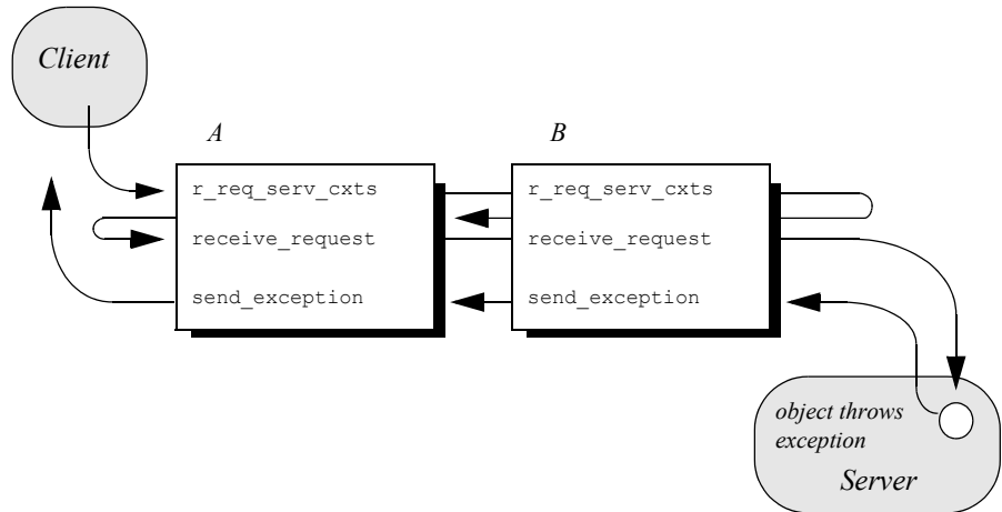
Figure 46 Server interceptors receive request and send exception thrown by target object.
