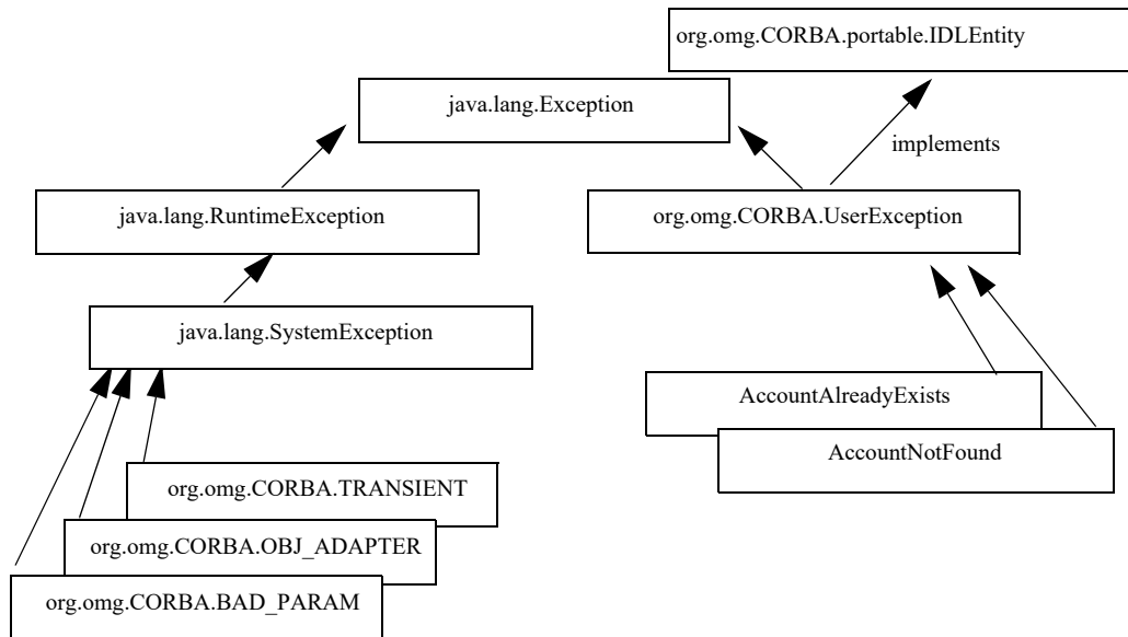
Figure 21 The Java mapping arranges exceptions into a hierarchy
