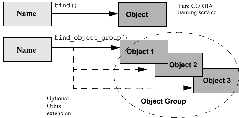
Figure 32 Associating a name with an object group
