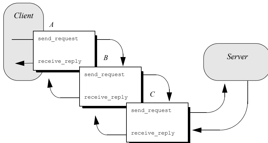
Figure 42 Client interceptors process a normal reply.
