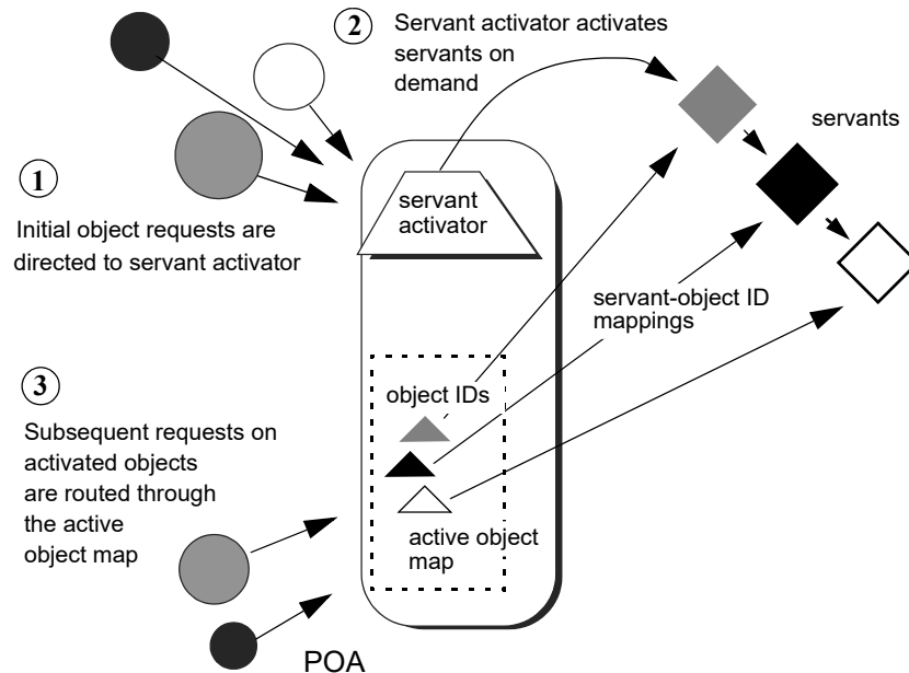
Figure 19 On the first request on an object, the servant activator returns a servant to the POA, which establishes the mapping in its active object map.
