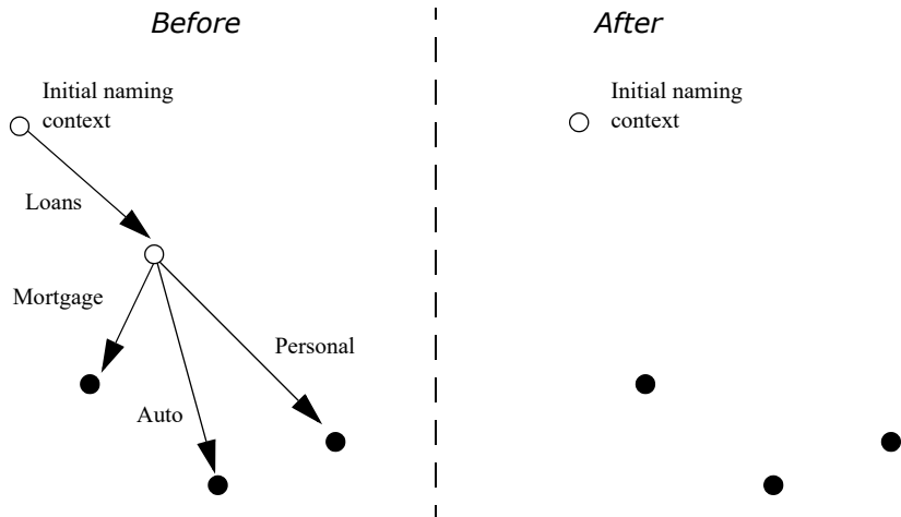
Figure 28 Destroying a naming context and removing related bindings
