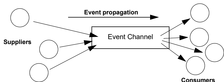
Figure 34 Suppliers and consumers communicating through an event channel
