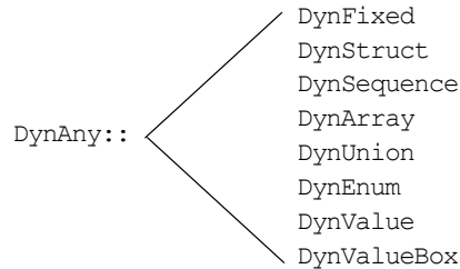
Figure 22 Interfaces that derive from the DynAny interface
