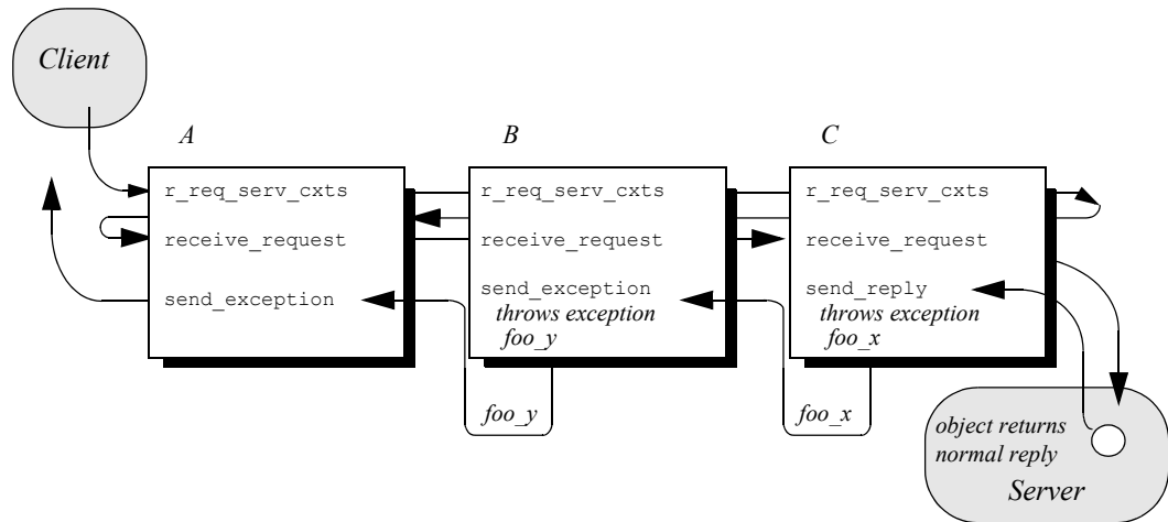
Figure 48 Server interceptors can change the reply type.
