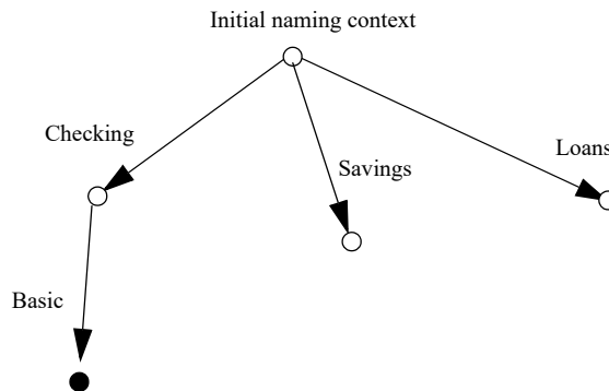
Figure 27 Binding an object reference to a naming context
