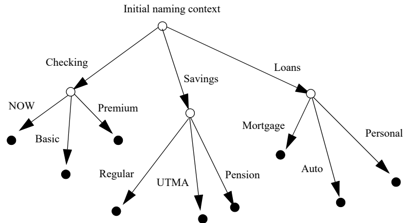
Figure 24 A naming graph is a hierarchy of naming contexts
