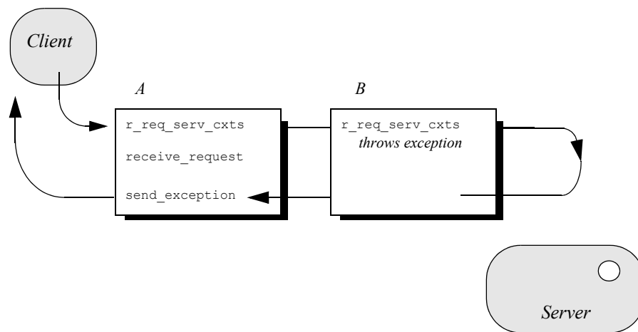
Figure 47 receive_request_service_contexts throws an exception and interception flow is aborted.
