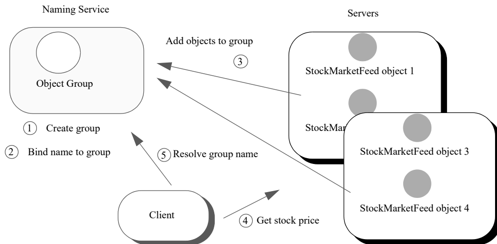
Figure 33 Architecture of the stock market example
