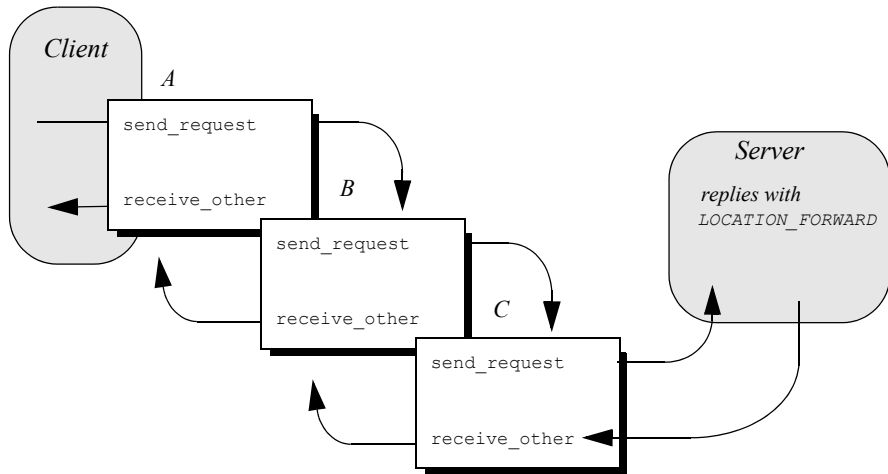
Figure 43 Client interceptors process a LOCATION_FORWARD reply.
