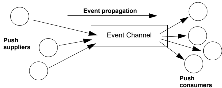
Figure 36 Push model of event transfer
