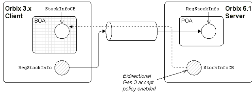
Figure 51 Orbix 3 Client Receiving a Callback from an Orbix 6.1 Server
