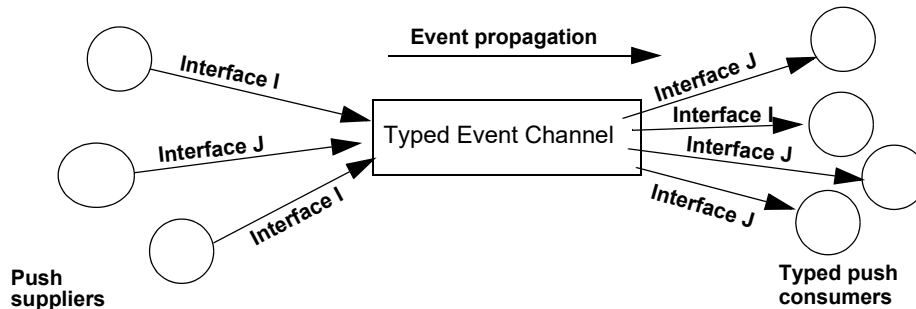
Figure 39 Push consumers pushing typed events to typed push consumers
