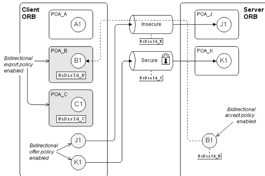
Figure 50 Advanced Bidirectional GIOP Scenario
