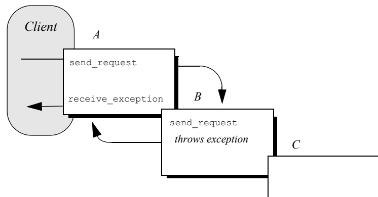
Figure 44 send_request throws an exception in a client-side interceptor
