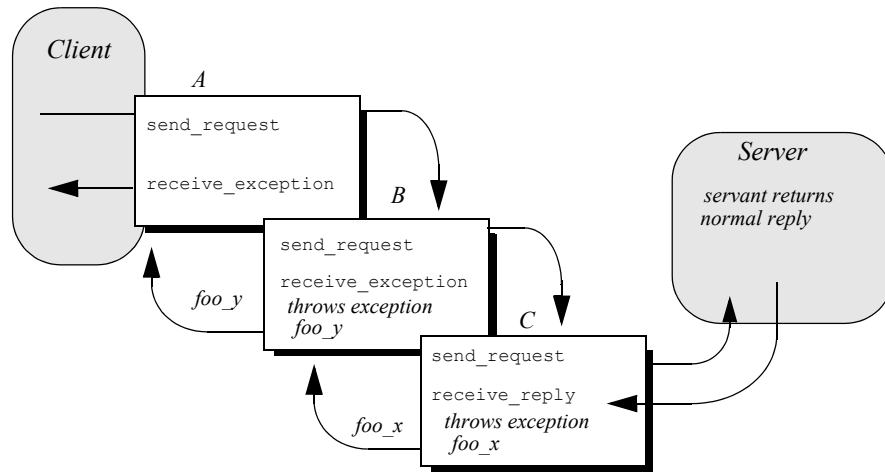
Figure 45 Client interceptors can change the nature of the reply.
