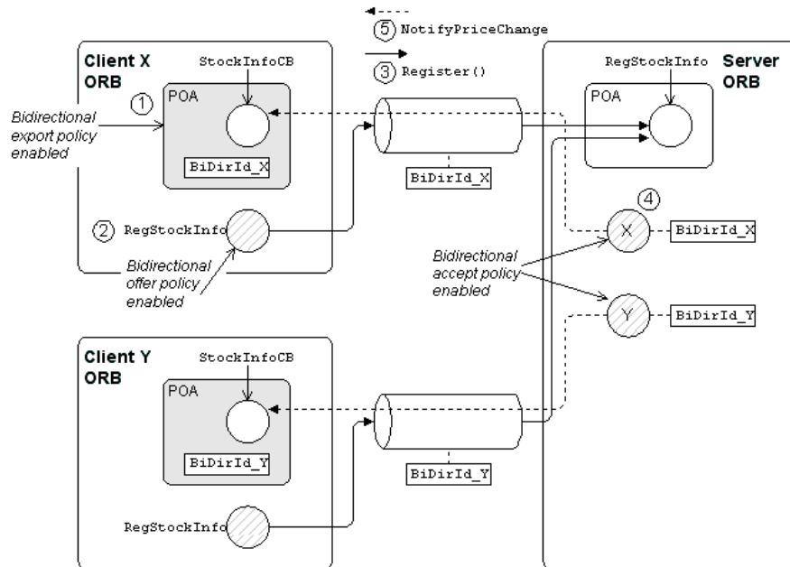
Figure 49 Basic Bidirectional GIOP Scenario—Stock Feed
