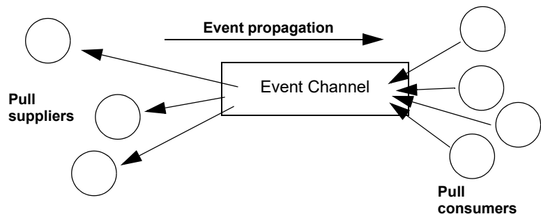
Figure 37 Pull Model suppliers and consumers communicating through an event channel
