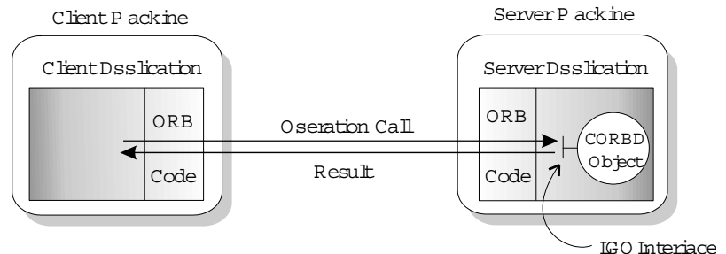
Figure 14 Client makes a single operation call on a server
