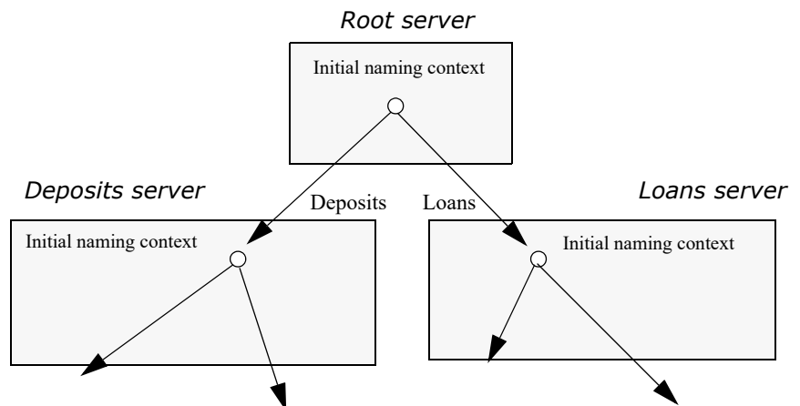
Figure 30 Multiple naming graphs are linked by binding initial naming contexts of several servers to a root server.
