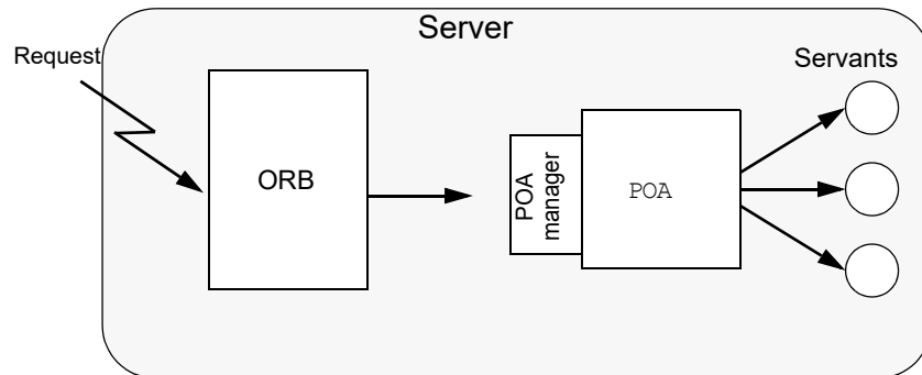
Figure 17 The server-side ORB conveys client requests to the POA via its manager, and the POA dispatches the request to the appropriate servant.
