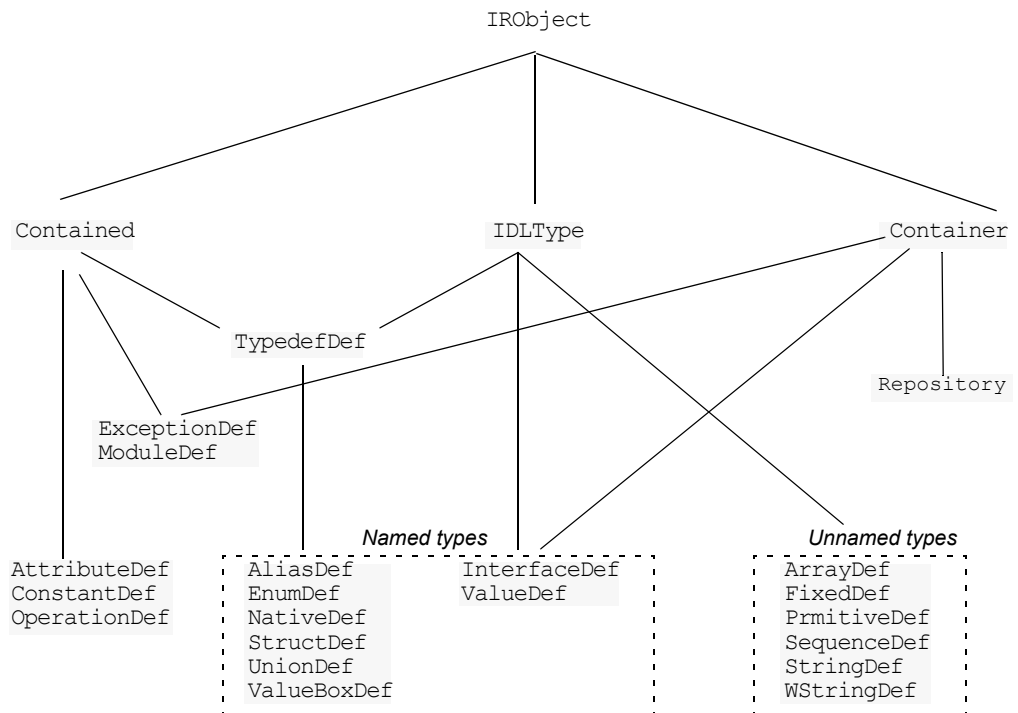
Figure 23 Hierarchy of interface repository objects
