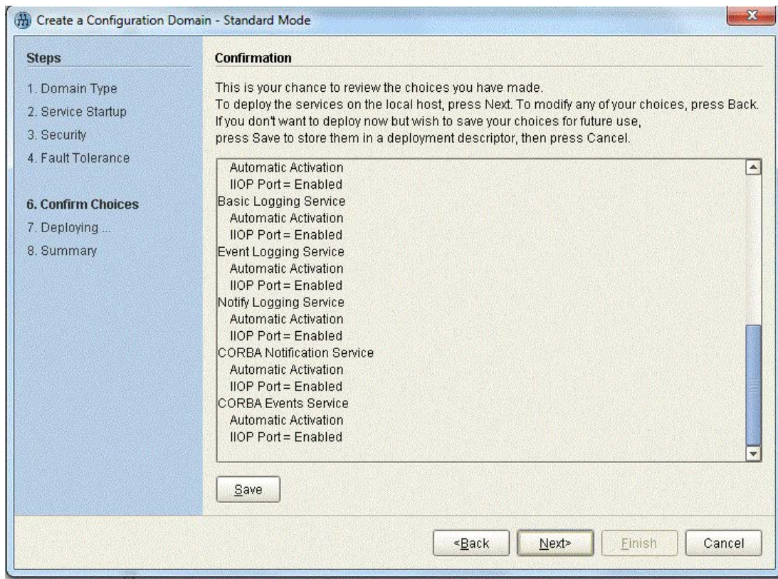
Figure 12 The Confirm Choices Window
