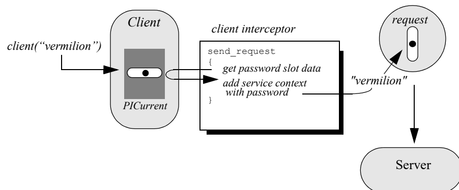
Figure 41 PICurrent facilitates transfer of thread context data to a request or reply.
