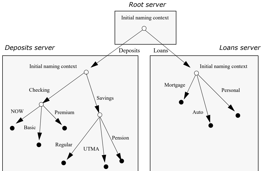
Figure 29 A naming graph that spans multiple servers
