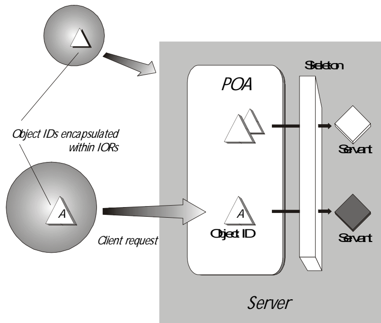
Figure 18 A portable object adapter (POA) maps abstract objects to their concrete implementations (servants)
