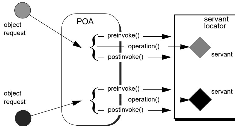
Figure 20 The POA directs each object request to the servant locator, which returns a servant to the POA to process the request.
