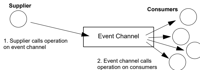
Figure 35 Event propagation in a CORBA system
