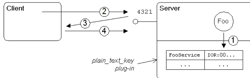
Figure 53 Using corbaloc with the plain_text_key Plug-In
