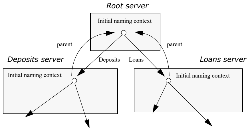
Figure 31 The root server's initial naming context is bound to the initial naming contexts of other servers, allowing clients to locate the root naming context.
