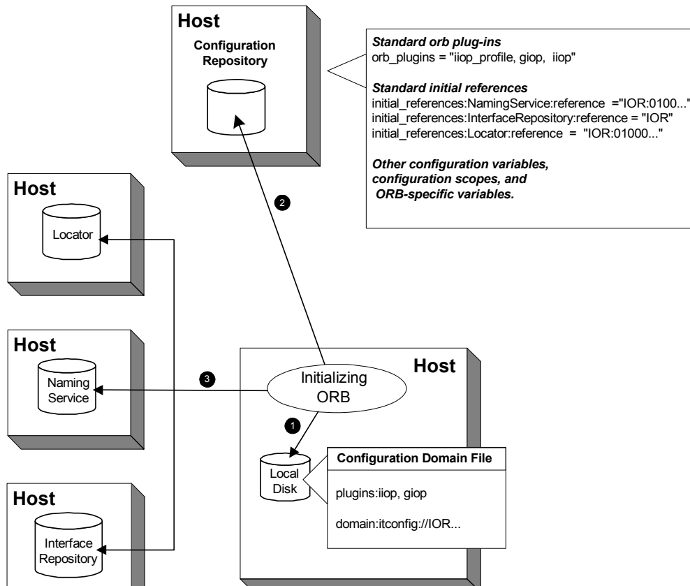
Figure 12 How an Orbix Application Obtains its Configurations
