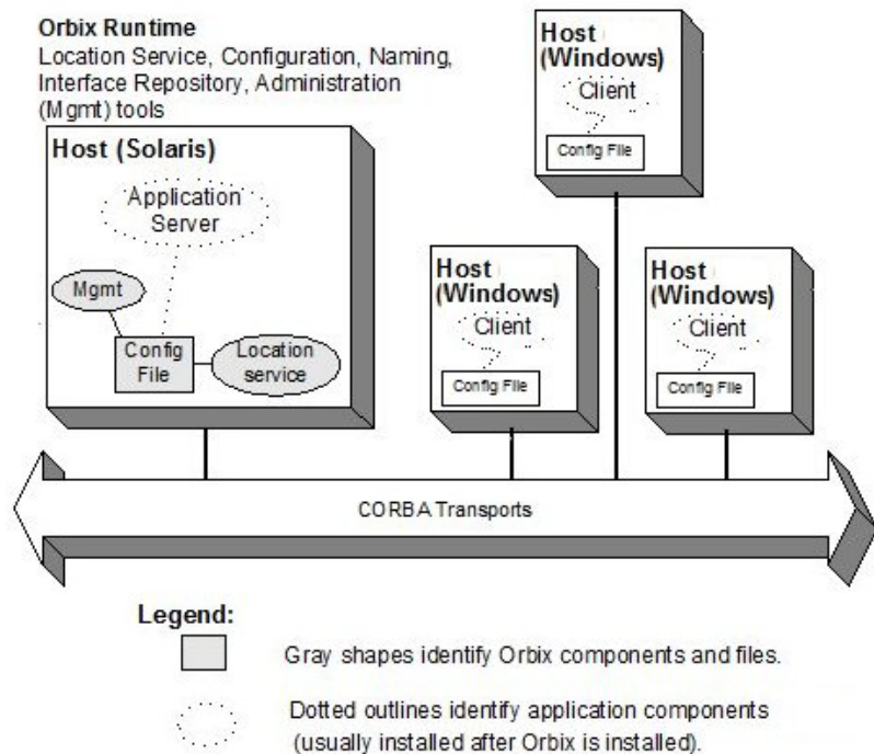
Figure 10 Orbix Environment with Local Configuration
