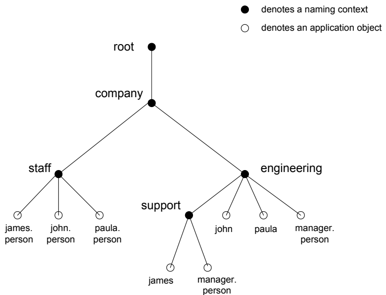
Figure 17 Naming Context Graph
