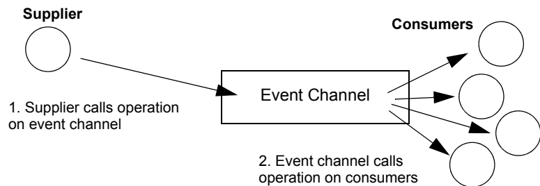
Figure 34: Event propagation in a CORBA system
