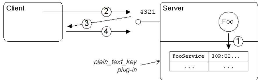
Figure 52: Using corbaloc with the plain_text_key Plug-In
