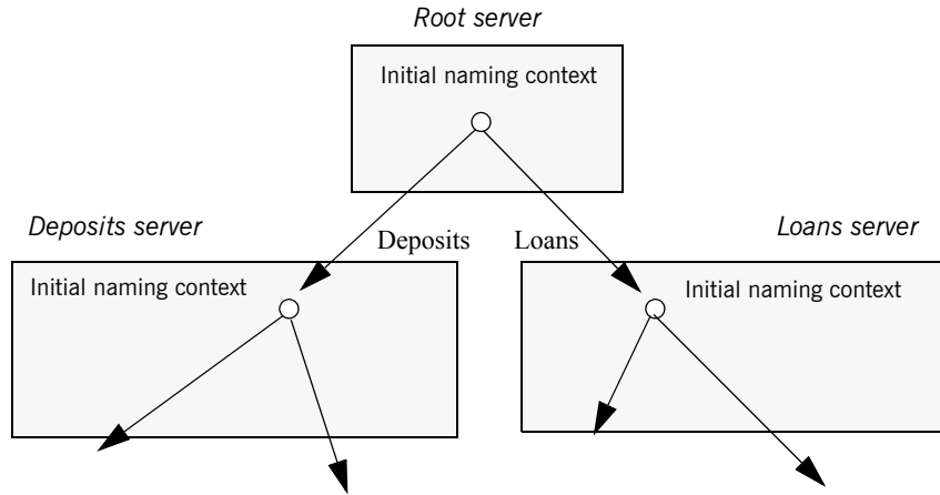
Figure 29: Multiple naming graphs are linked by binding initial naming contexts of several servers to a root server.
