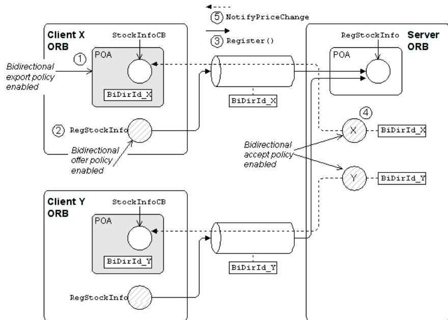
Figure 48: Basic Bidirectional GIOP Scenario—Stock Feed
