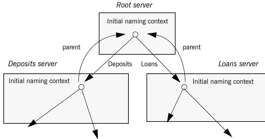
Figure 30: The root server's initial naming context is bound to the initial naming contexts of other servers, allowing clients to locate the root naming context.
