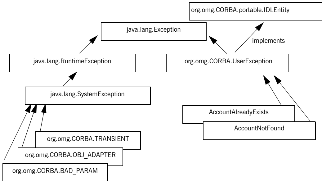
Figure 20: The Java mapping arranges exceptions into a hierarchy
