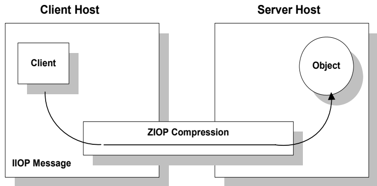
Figure 53: Overview of ZIOP Compression
