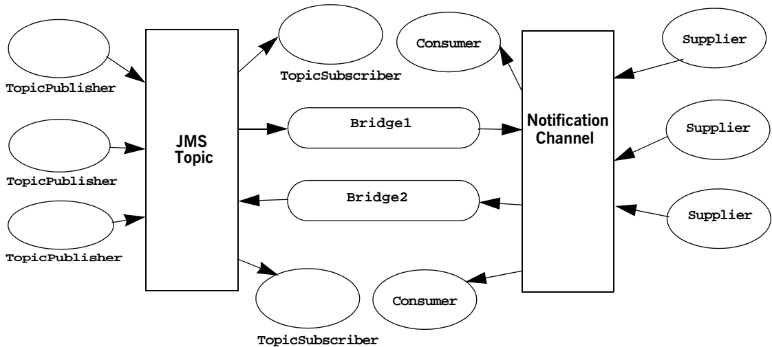
Figure 7: JMS-Notification Bridging
