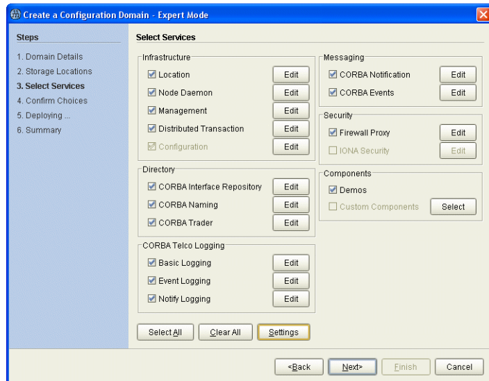
Figure 7: Selecting Services
