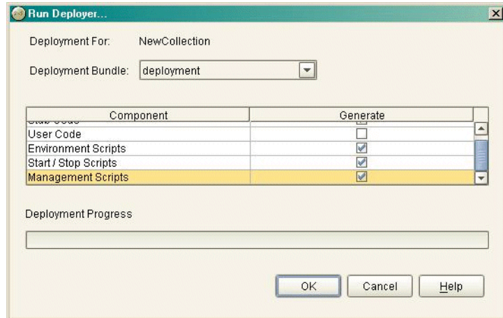
Figure 4: Run Deployer Dialog
