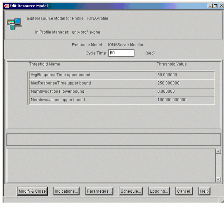
Figure 9: Edit Resource Model
