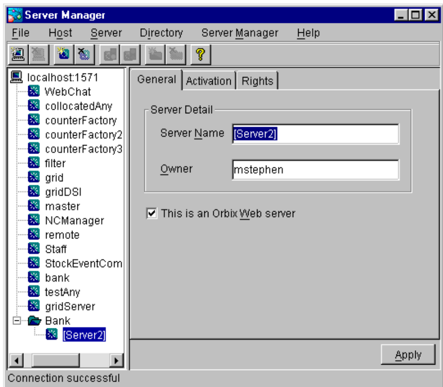
Figure 14: Registering a New Server
