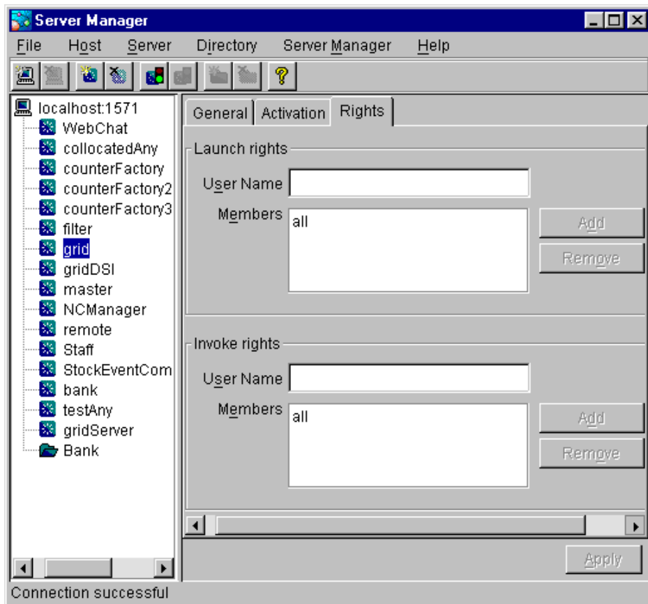
Figure 15: Providing Server Access Rights
