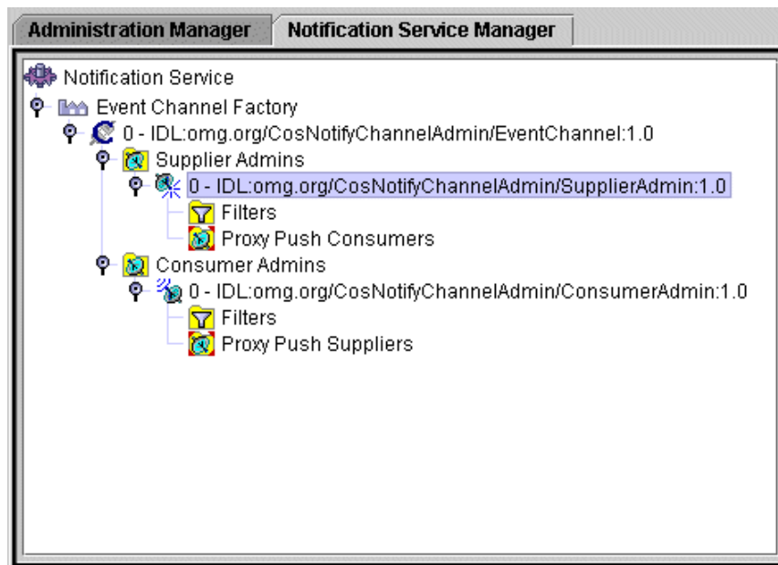
Figure 16 Proxy Objects
