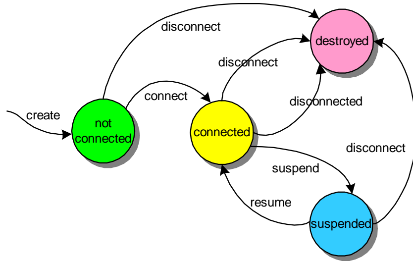
Figure 4 Proxy States
