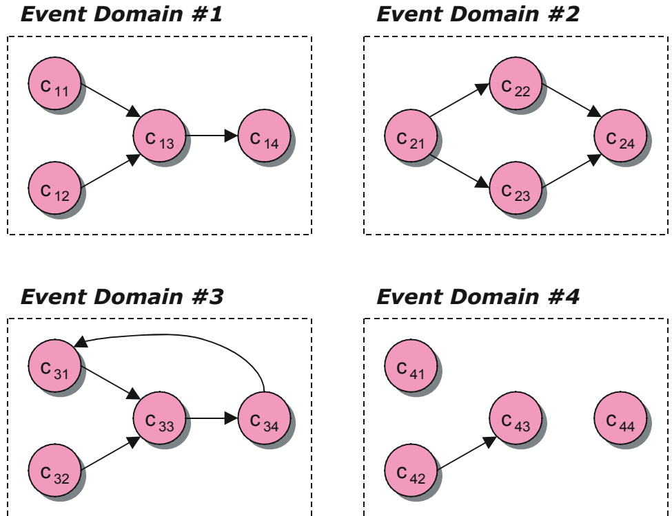
Figure 13 Different Types of Event Domains
