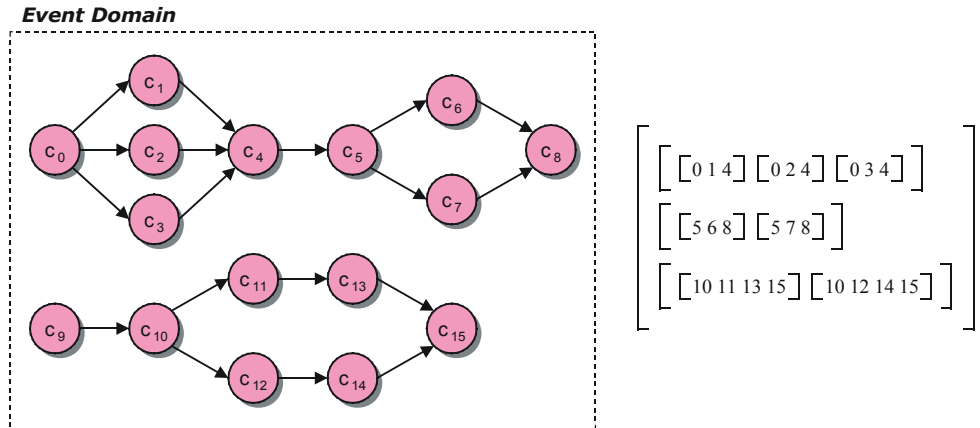
Figure 16 Domain Containing Three Diamonds
