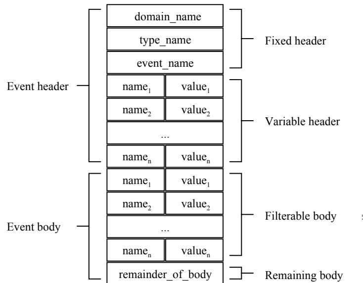
Figure 3 Structured Event
