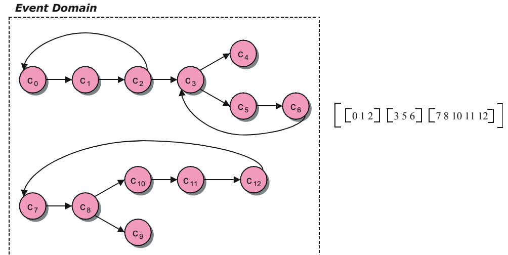
Figure 15 Domain Containing Three Cycles
