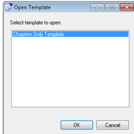
Figure 12-2. Open Template
