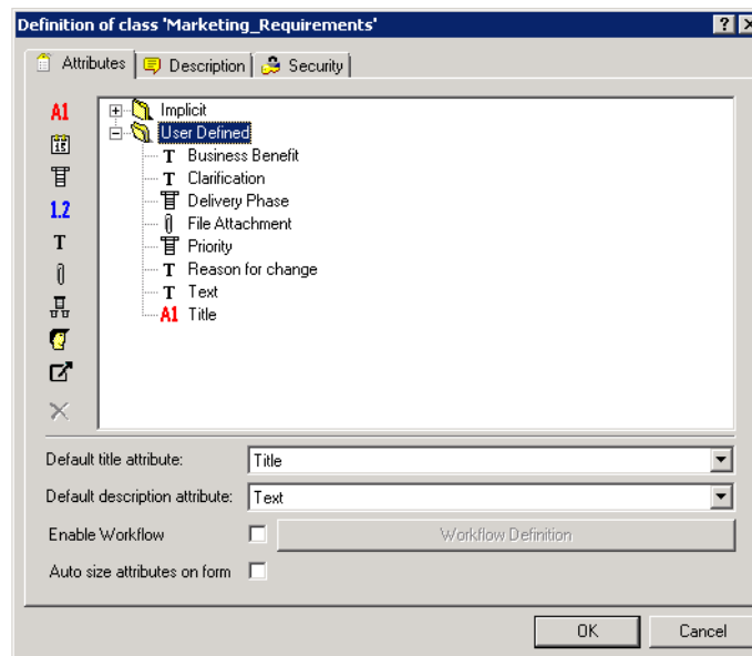
Figure 9-15. Class Definition
