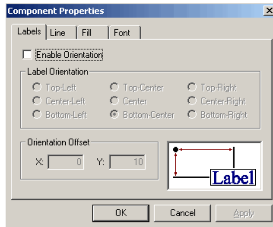
Figure 9-14. Component Properties
