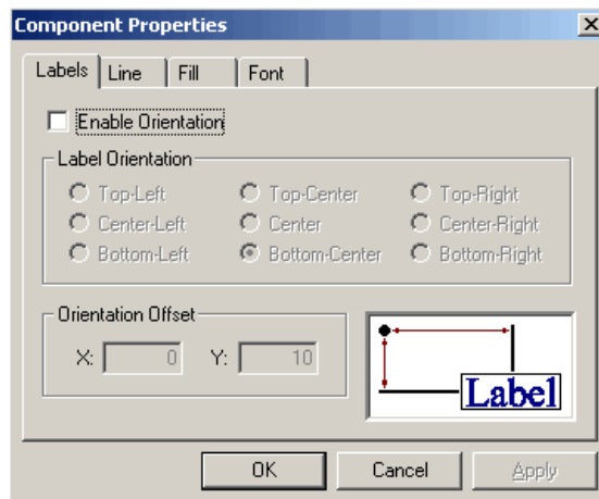
Figure 9-17. Component Properties
