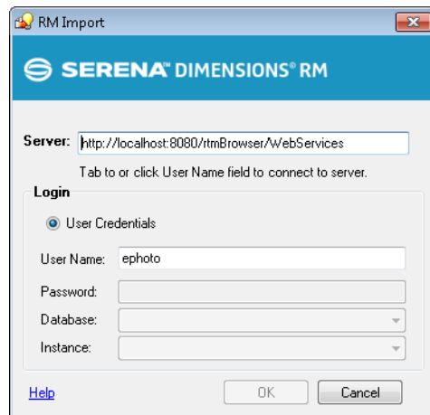
Figure 12-1. Login Dialog
