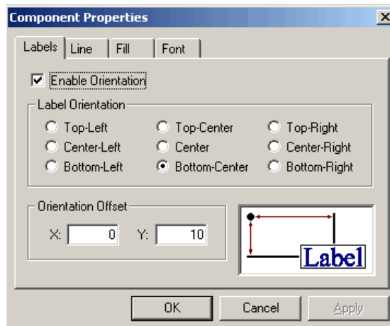
Figure 9-23. Component Properties
