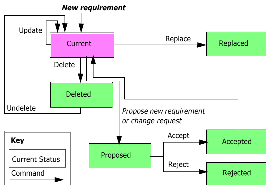
Figure 1-6. Object Lifecycle
