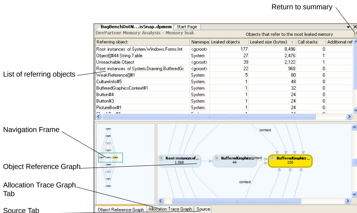
Figure 5-5. DevPartner Memory Analysis - memory leaks object reference details
