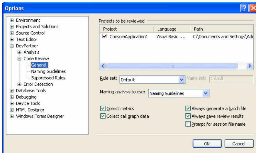
Figure 3-4. General options page
