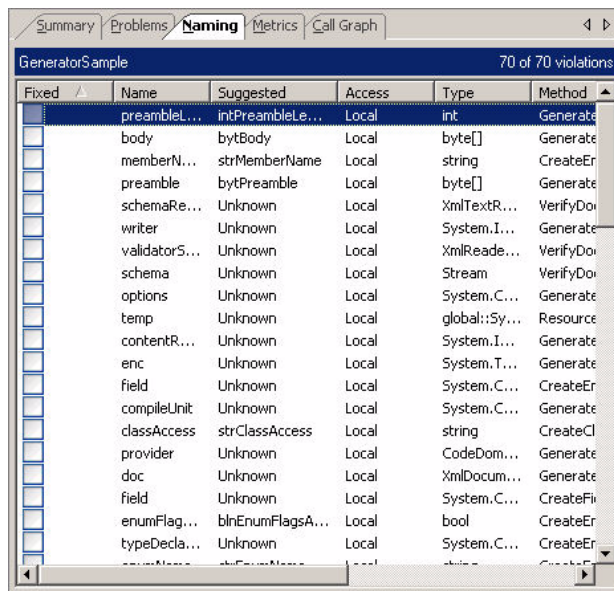
Figure 3-3. Naming tab and Details pane
