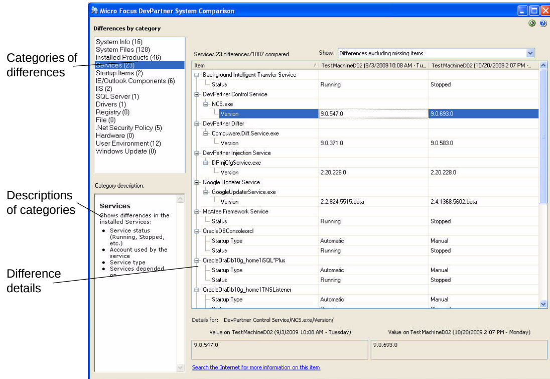
Figure 8-3. Results window
