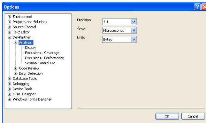
Figure 5-10. Analysis Options
