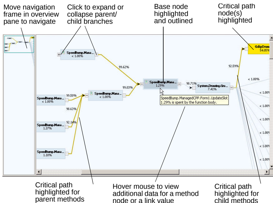
Figure 6-10. Call graph
