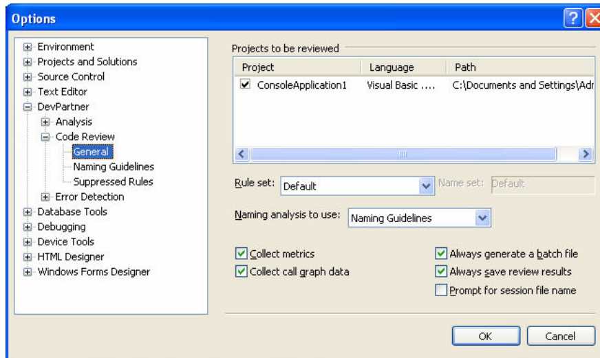
Figure 3-1. DevPartner Code Review general options
