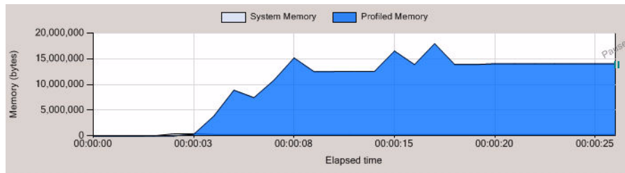
Figure 5-24. Real-time graph suggesting excessive temporary object creation
