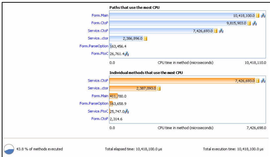
Figure 7-2. The Performance Expert Results Summary
