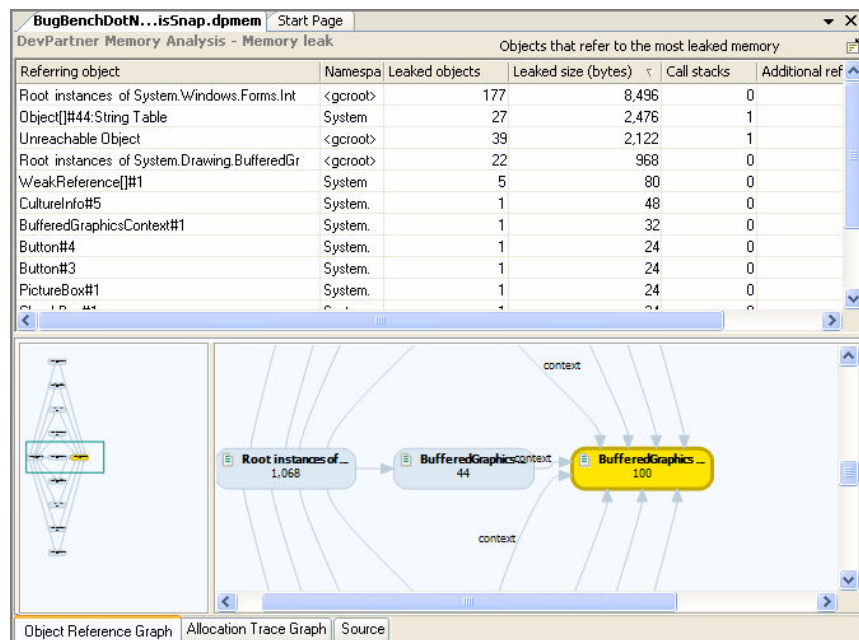
Figure 5-13. Memory Analysis Object Reference graph
