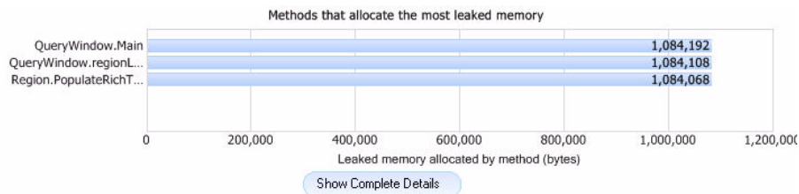
Figure 5-22. Methods that allocate the most leaked memory
