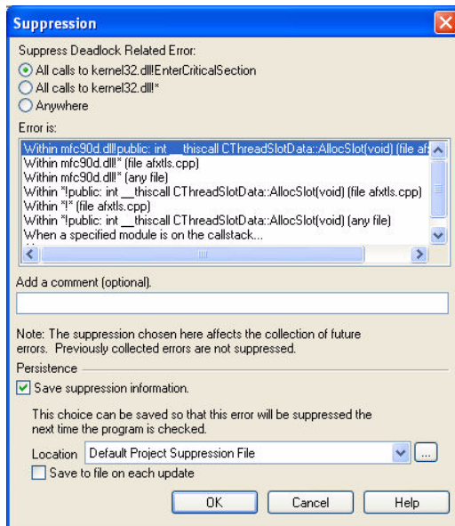
Figure 2-6. The Suppression dialog box
