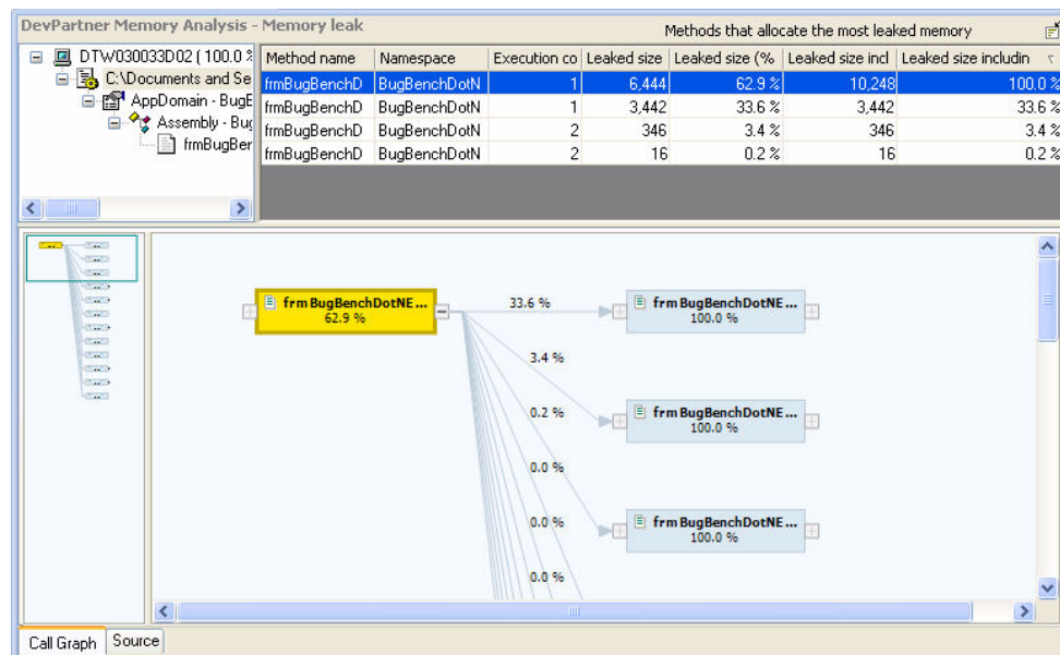
Figure 5-14. Memory Analysis Call graph
