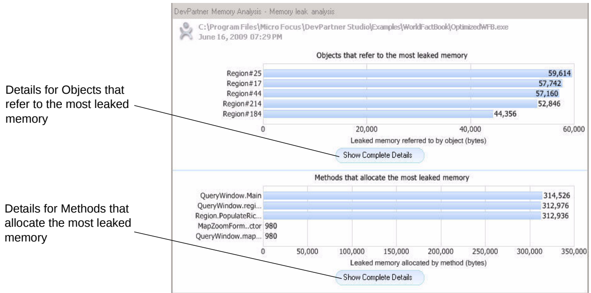
Figure 5-4. DevPartner Memory Analysis - Memory Leaks Analysis summary
