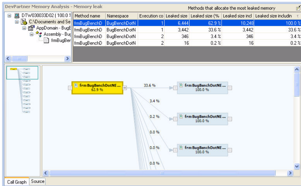
Figure 5-23. Details for methods that allocate the most leaked memory
