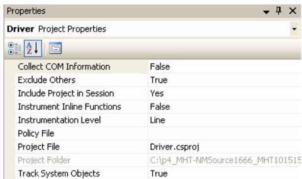
Figure 6-6. Project properties
