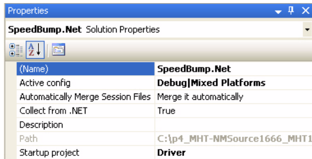
Figure 6-5. Solution properties
