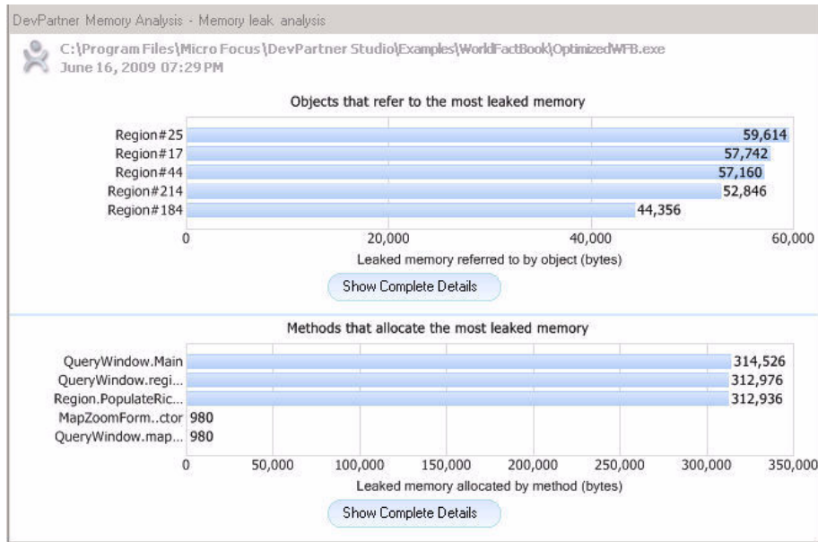
Figure 5-18. Results Summary appears when you click View Memory Leaks
