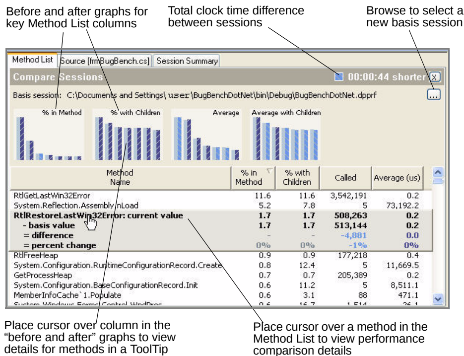
Figure 6-11. Comparing performance sessions
