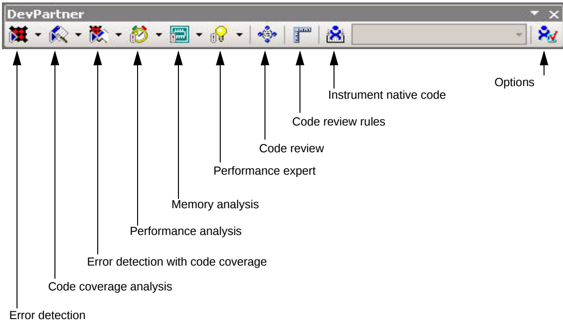
Figure 1-1. DevPartner toolbar
