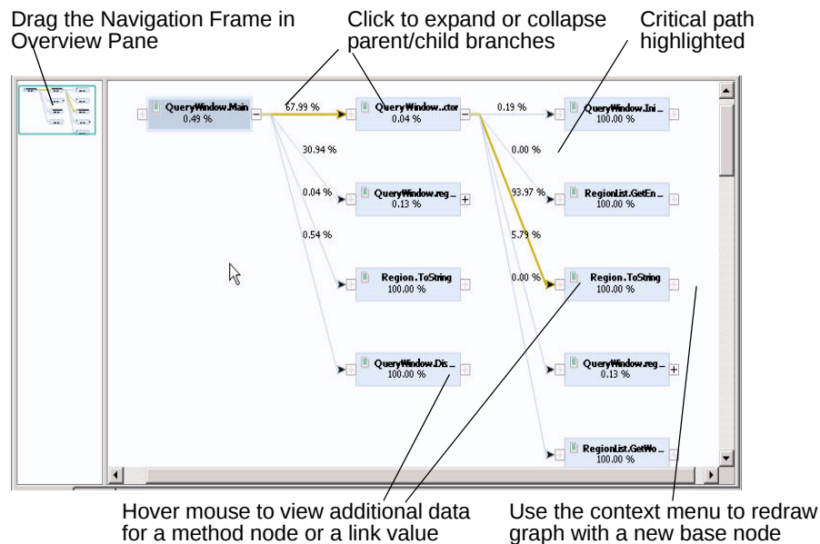
Figure 5-25. A Call graph for an entry point method shows the critical path
