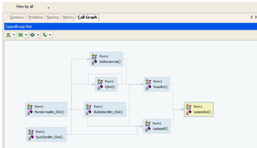
Figure 3-12. Call Graph tab showing example of Call Graph representation
