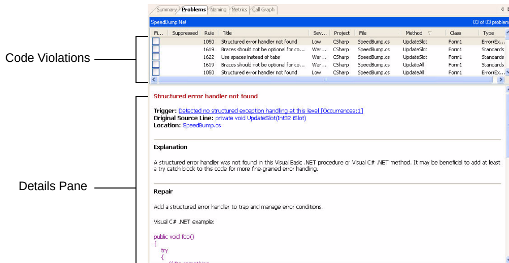
Figure 3-8. Problems tab and Details pane
