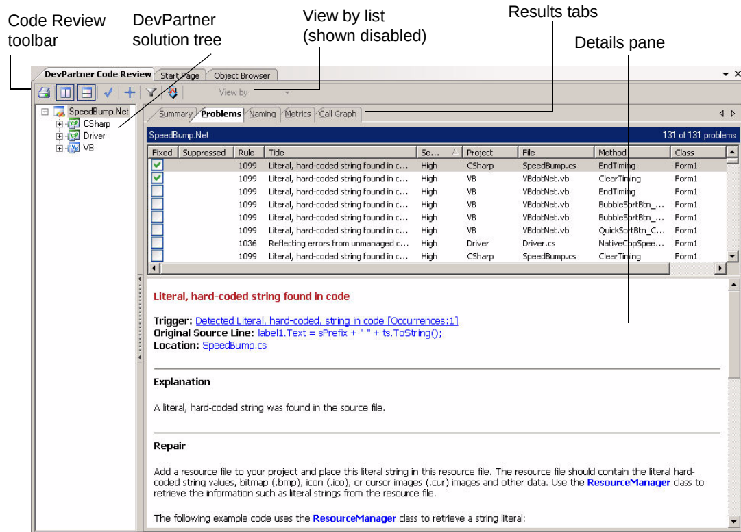
Figure 3-2. Code Review Results window
