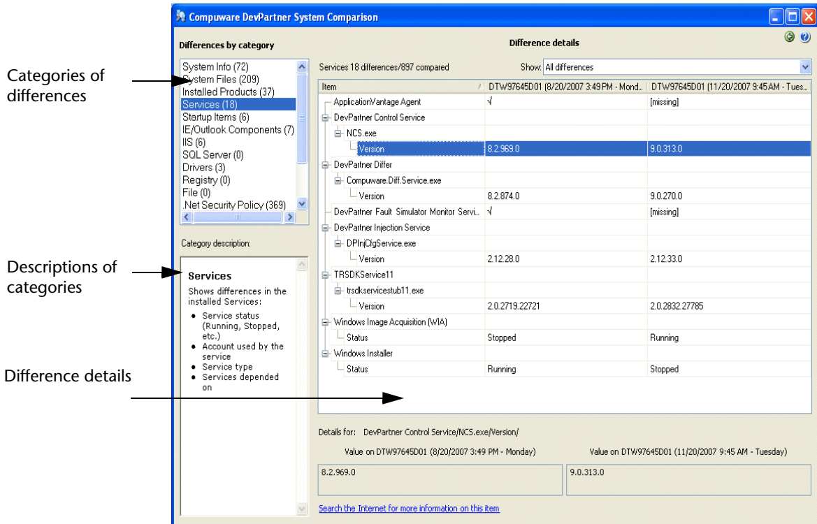
Figure 8-3. Results Window
