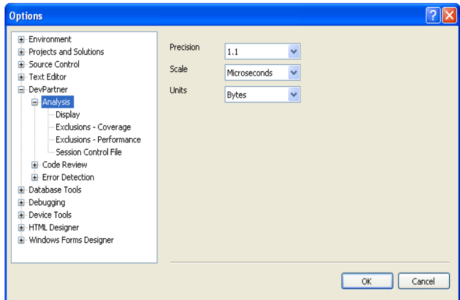
Figure 4-6. Analysis Options
