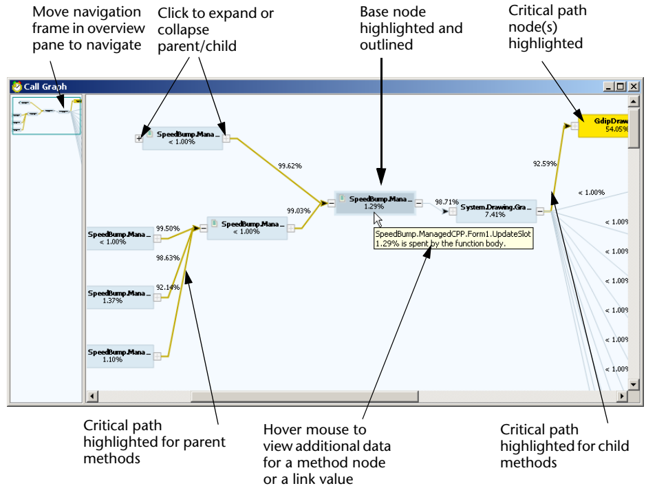
Figure 6-11. Call Graph
