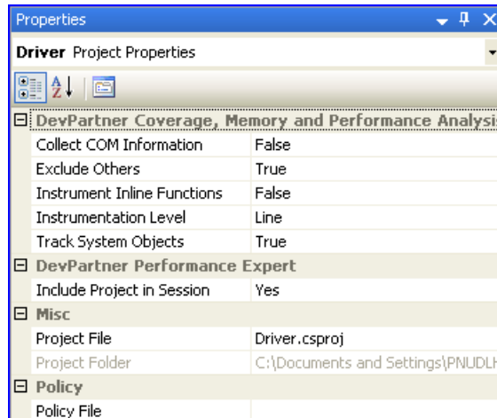
Figure 4-5. Project Properties
