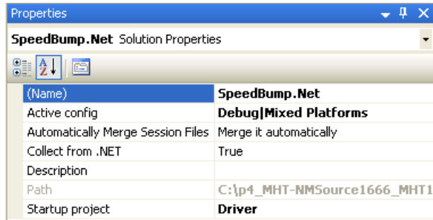
Figure 7-9. Solution Properties
