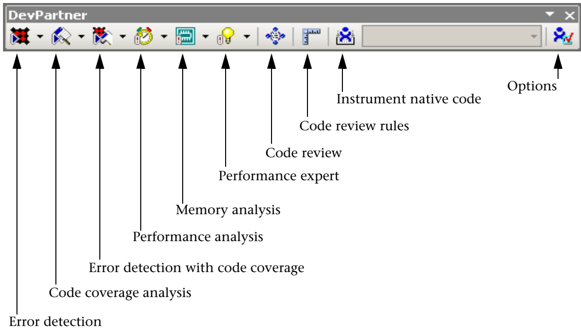
Figure 1-1. DevPartner Toolbar
