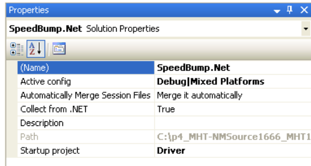
Figure 5-8. Solution Properties
