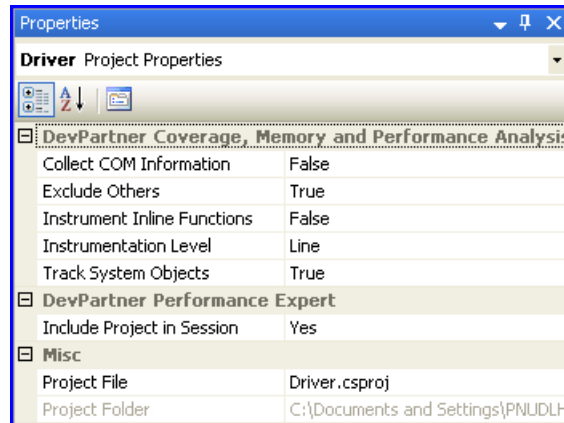
Figure 5-9. Project Properties
