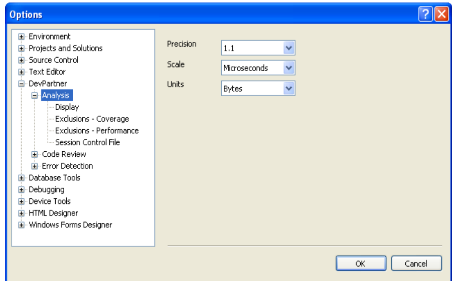
Figure 6-7. Analysis Options
