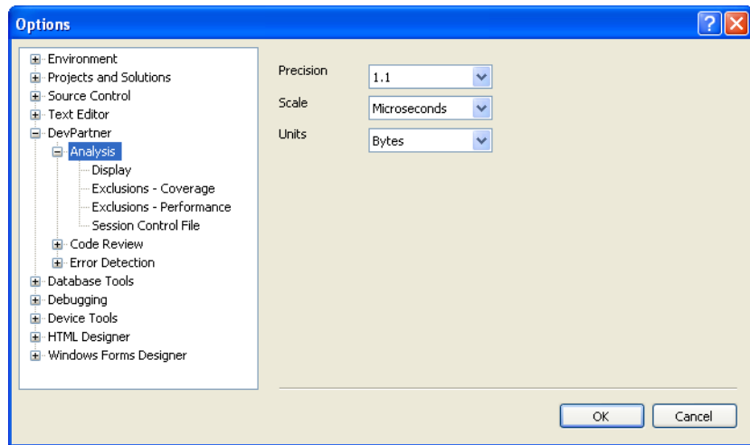
Figure 7-11. Analysis Options
