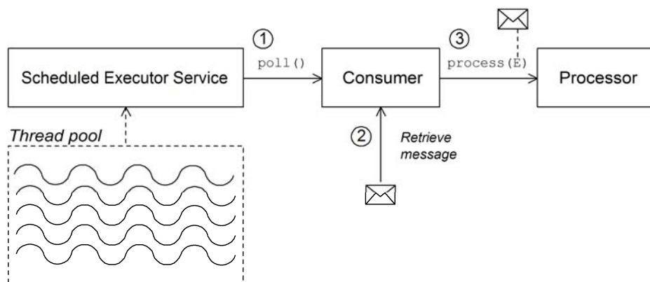
Figure 8. Scheduled Poll Consumer
