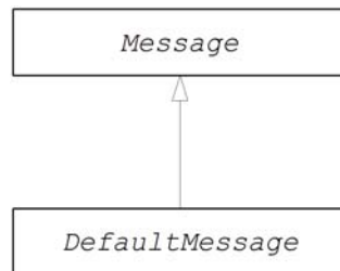
Figure 17. Message Inheritance Hierarchy
