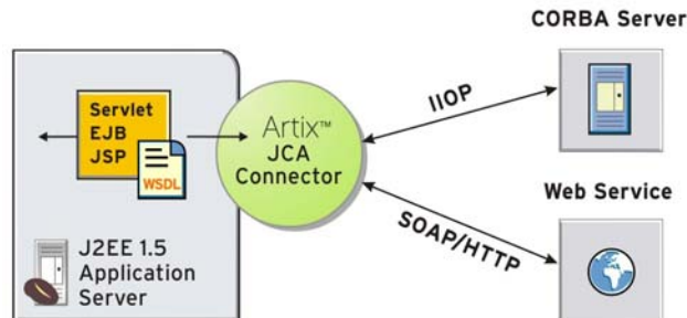
Figure 1. Connecting J2EE Applications to Web services
