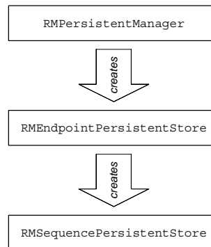
Figure 20: Overview of the WS-RM Persistence API
