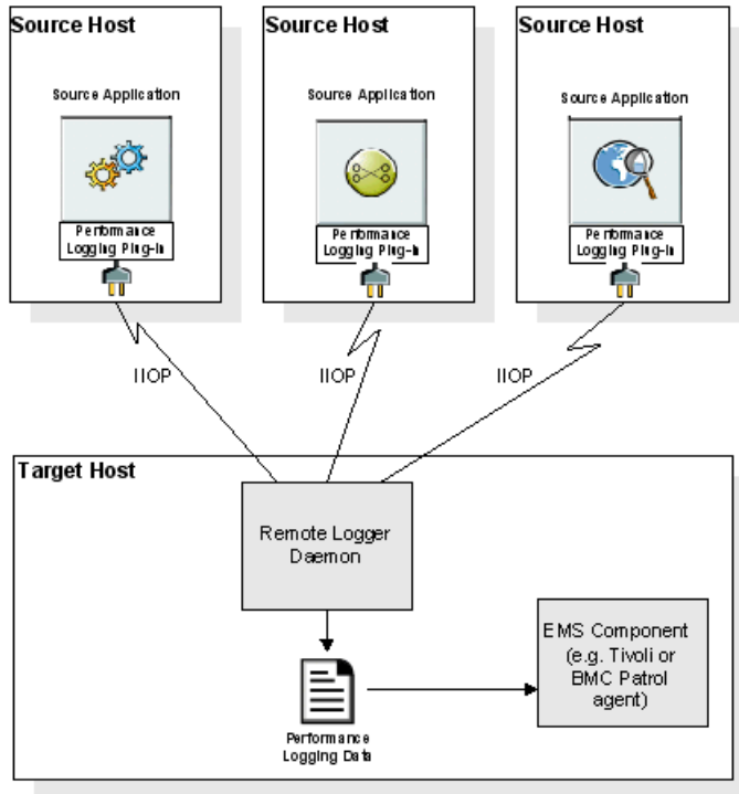
Figure 2: Remote Logging Framework
