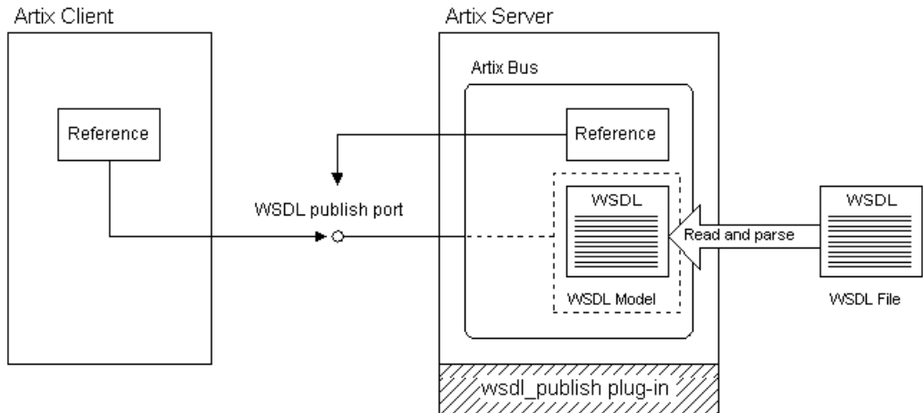
Figure 16: Creating References with the WSDL Publishing Service
