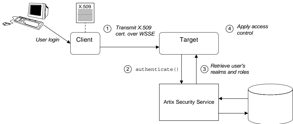
Figure 13: Overview of Certificate-Based Authentication with WSS
