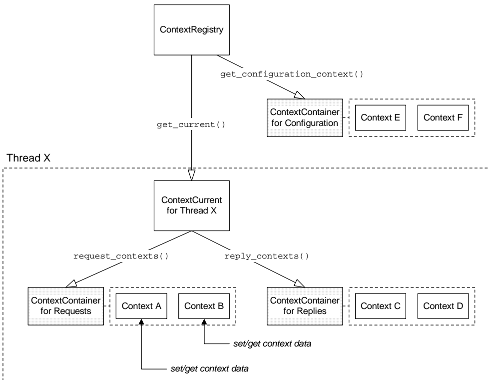
Figure 21: Overview of the Context Architecture
