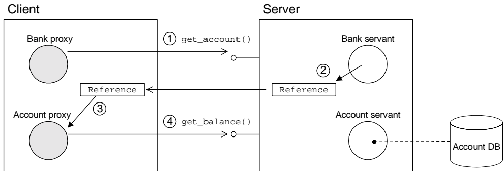
Figure 14: Using Bank to Obtain a Reference to an Account
