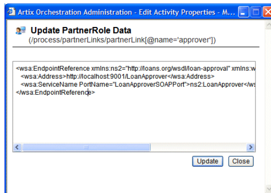
Figure 9: The Update Partner Role Data Dialog
