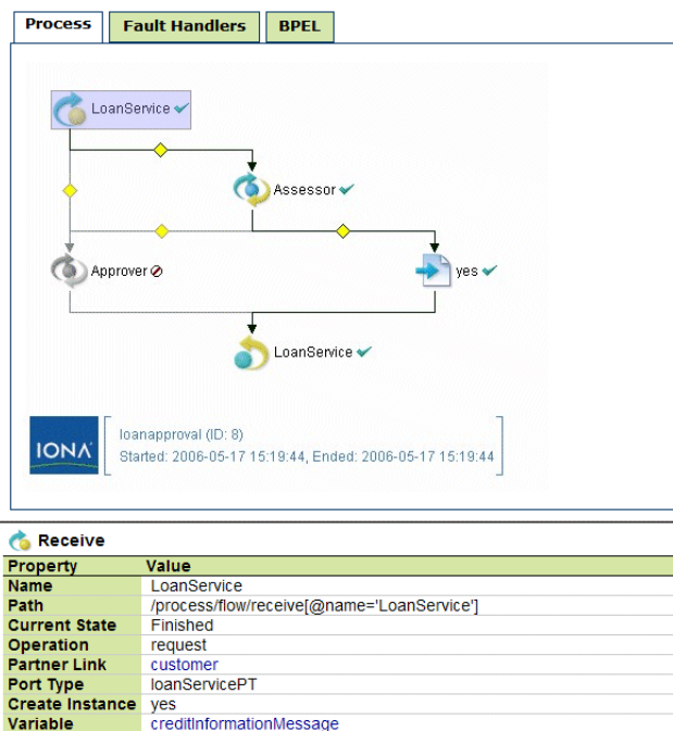
Figure 3: Active Process Details Graphic View
